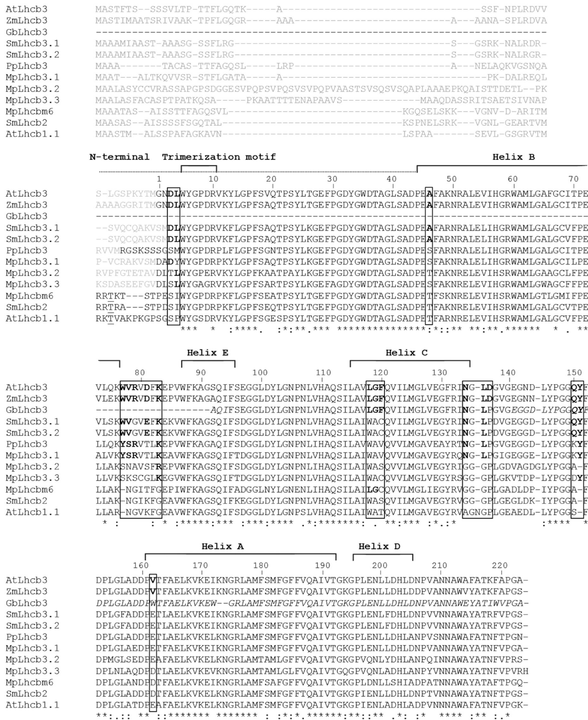
Fig. (4). Determination of Lhcb3-specific amino acids. All Lhcb3 sequences were aligned; two phylogenetically closest sequences, MpLhcbm6 and SmLhcb2, as well as AtLhcb1.1 were also added for comparison. Amino acids numbers are based on AtLhcb3 sequence. Light grey: signal peptide. Underlined: phosphorylatable threonine. Bold and in boxes: specific amino acids of Lhcb3, based on angiosperms sequences. GbLhcb3 is incomplete in the EST database, and was partially completed (residues in italics) with the sequence determined in [30]. Abbreviations of plant species are as in Fig. 2.
