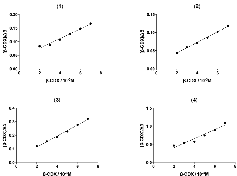
Figure SI2. Representation of the ligand: \beta CD interaction (Scott plots). [Ligand] = 0.5 \cdot 10^{-3}\text{M} , [ \beta CD] = 2\text{-}7 \cdot 10^{-3}\text{M} .
