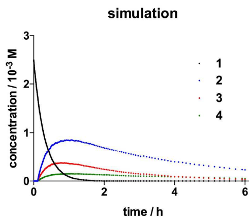
Figure SI1. Simulation of the formation of lignans from the oxidation of coniferyl alcohol. Stochastic calculations performed with the freeware Kinetiscope. Initial parameters: [\mathbf{1}] = 2.5 \cdot 10^{-3} \text{M} , k_1 = 3.3 \text{ h}^{-1} ; k_2 = 0.3 \text{ h}^{-1} ; k_3 = 0.5 \text{ h}^{-1} ; k_4 = 0.25 \text{ h}^{-1} .
