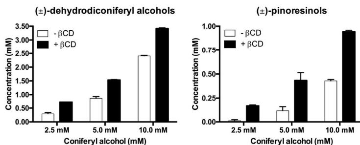
Figure SI6. Effects of a variable initial concentrations of coniferyl alcohol on the formation of dimers in the presence of βCD.
