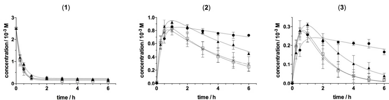
Figure 1. Influence of CDs on the laccase catalysed oxidation of coniferyl alcohol. Coniferyl alcohol ( 1 ) ( 2.5 \times 10^{-3} M) was incubated with the laccase LAC3 ( 5 \text{ U.L}^{-1} ) at 30^\circ\text{C} in the absence (open square) or presence of an excess ( 12 \times 10^{-3} M) of either \alpha CD (crosses), \beta CD (black circles) or \gamma CD (black triangles). Consumption of 1 and apparition of 2 and 3 were monitored by RP-
