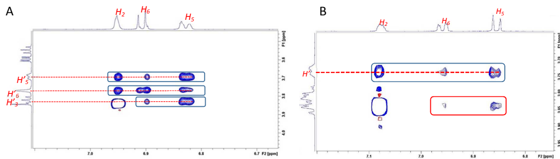
Figure SI.4. Fragments of ROESY spectra showing the intermolecular interactions between protons from ligands and proton from \beta -CD. Panel A, ligand = ( \pm )-pinoresinol; panel B, ligand = coniferyl alcohol.
