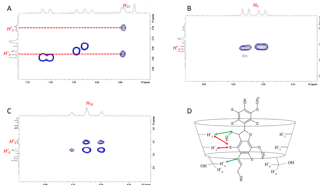
Figure S15. Fragments of ROESY spectra showing the intermolecular interactions between protons from dehydro di-coniferyl alcohol and proton from βCD. Panel A, zoom in the interactions between the proton H 15 of dehydro di-coniferyl alcohol and protons H' 3 and H' 5 of βCD; panel B, zoom in the interactions between the proton H 9 of dehydro di-coniferyl alcohol and protons H' 3 of βCD (figure panel D); panel C, zoom in the interactions between the proton H 16 of dehydro di-coniferyl alcohol and protons H' 5 and H' 6 of βCD (figure panel D); panel D, scheme of the potential interactions; double arrows indicate spatial dipolar interactions classified from each CD proton: close (red), intermediate (green).
