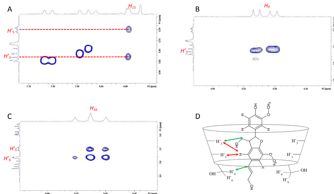
Figure SI5. Fragments of ROESY spectra showing the intermolecular interactions between protons from dehydro di-coniferyl alcohol and proton from βCD. Panel A, zoom in the interactions between the proton H 15 of dehydro di-coniferyl alcohol and protons H' 3 and H' 5 of βCD; panel B, zoom in the interactions between the proton H 9 of dehydro di-coniferyl alcohol and protons H' 3 of βCD (figure panel D); panel C, zoom in the interactions between the proton H 16 of dehydro di-coniferyl alcohol and protons H' 5 and H' 6 of βCD (figure panel D); panel D, scheme of the potential interactions; double arrows indicate spatial dipolar interactions classified from each CD proton: close (red), intermediate (green).
