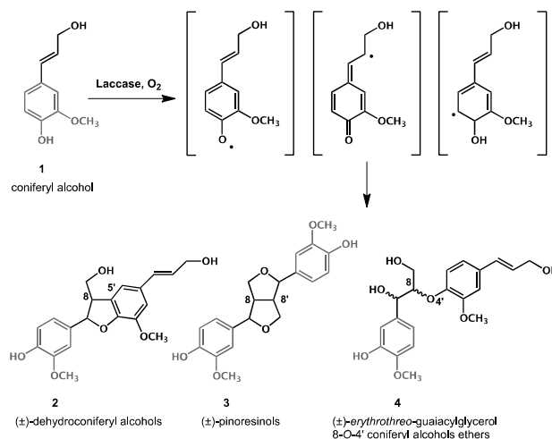
Scheme 1. Laccase catalysed oxidation of coniferyl alcohol
