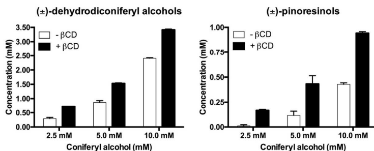
Figure S16. Effects of a variable initial concentrations of coniferyl alcohol on the formation of dimeric lignans in the presence of βCD.
