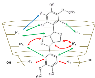
Figure 3. Schematic view of a potential \beta CD/( \pm )-pinoresinol inclusion complex as deduced from 2D-ROESY data. Double arrows indicate spatial dipolar interactions classified from each CD proton: close (red), intermediate (green), far (blue).
