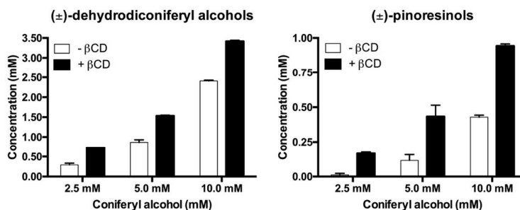
Figure SI6. Effects of a variable initial concentrations of coniferyl alcohol on the formation of dimers in the presence of \beta CD.
