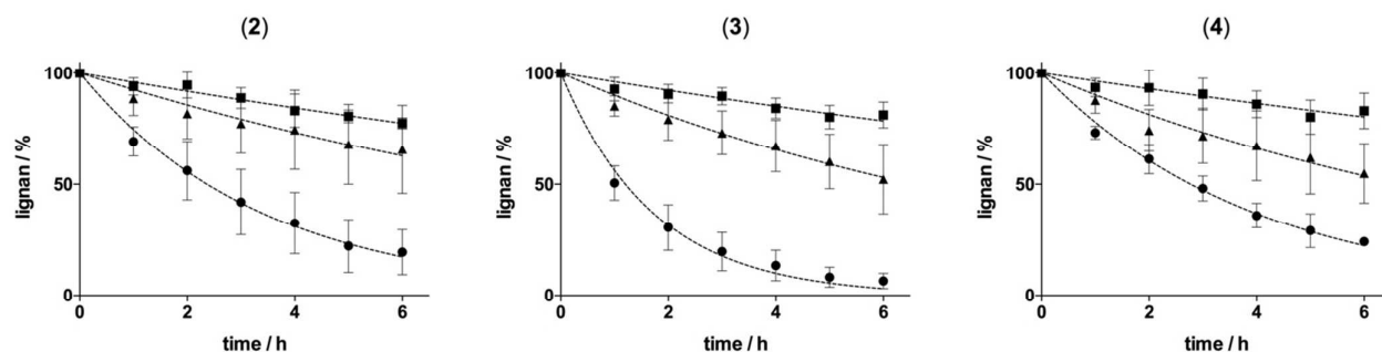
Figure 2. Influence of CDs on the laccase catalysed oxidation of lignans. Dehydroconiferyl alcohol (2), pinosresinol (3) or erythro guaiacyl glycerol (4) ( 2.5 \times 10^{-3} M) were each incubated with the laccase LAC3 ( 5 \text{ U.L}^{-1} ) at 30^\circ\text{C} in the absence (black circles) or presence of an excess ( 12 \times 10^{-3} M) of either \beta CD (black squares) or \gamma CD (black triangles). Oxidations were monitored by RP-HPLC. Fits (dashed lines) were obtained using a single decay (exponential) model.
