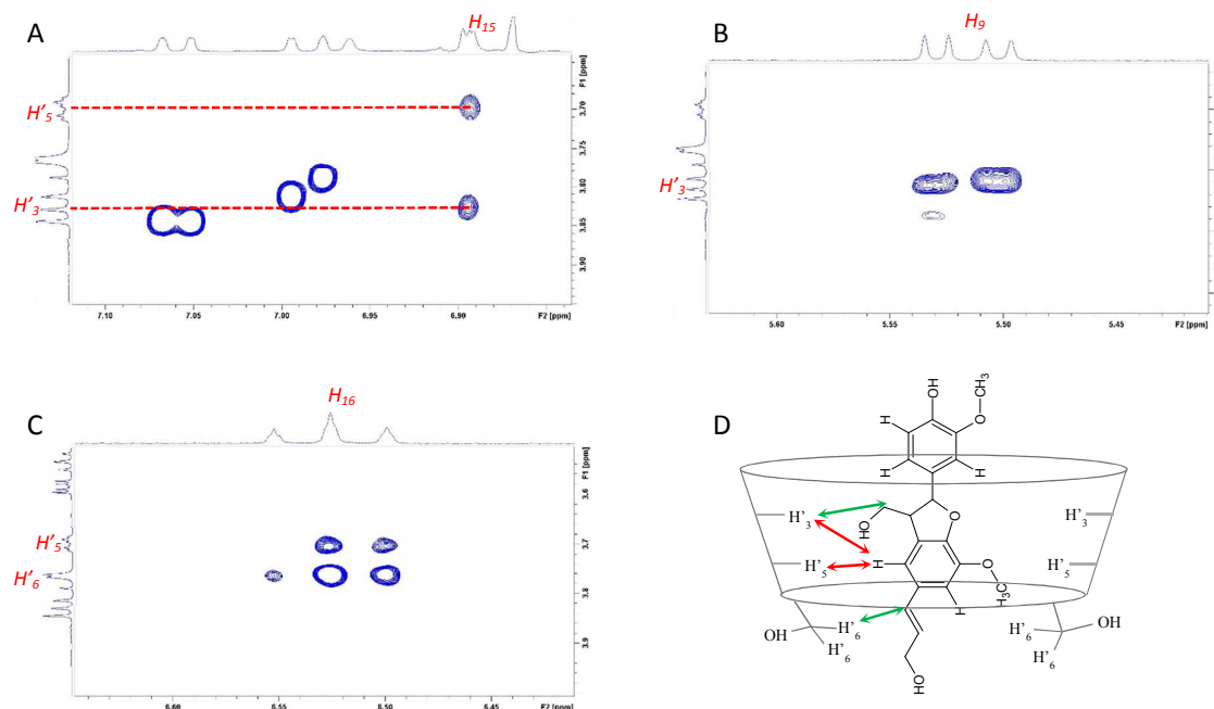
Figure SI5. Fragments of ROESY spectra showing the intermolecular interactions between protons from dehydro di-coniferyl alcohol and proton from \beta CD. Panel A, zoom in the interactions between the proton H 15 of dehydro di-coniferyl alcohol and protons H' 3 and H' 5 of \beta CD; panel B, zoom in the interactions between the proton H 9 of dehydro di-coniferyl alcohol and protons H' 3 of \beta CD (figure panel D); panel C, zoom in the interactions between the proton H 16 of dehydro di-coniferyl alcohol and protons H' 5 and H' 6 of \beta CD (figure panel D); panel D, scheme of the potential interactions; double arrows indicate spatial dipolar interactions classified from each CD proton: close (red), intermediate (green).
