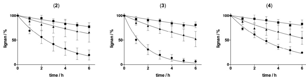
apparently no significant effect on the rate of oxidation of 1 and 4 , whereas they have a marked effect on the stabilization of 2, 3 . Figure 2. Influence of CDs on the laccase catalysed oxidation of the dimers 2, 3 and 4 . Dehydroconiferyl alcohol ( 2 ), pinosresinol ( 3 ) or erythro guaiacyl glycerol ( 4 ) ( 2.5 \times 10^{-3} M) were each incubated with the laccase LAC3 ( 5 \text{ U.L}^{-1} ) at 30^\circ\text{C} in the absence (black circles) or presence of an excess ( 12 \times 10^{-3} M) of either \beta CD (black squares) or \gamma CD (black triangles). Oxidations were monitored by RP-HPLC. Fits (dashed lines) were obtained using a single decay (exponential) model.
