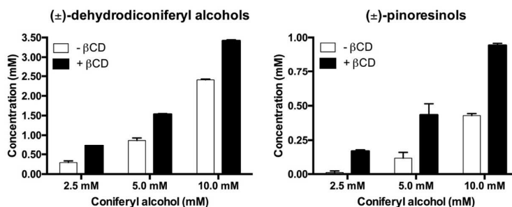
Figure S16. Effects of a variable initial concentrations of coniferyl alcohol on the formation of dimeric lignans in the presence of \beta CD.
