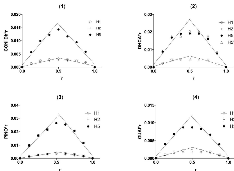
Figure S13. Representation of the ligand: \beta CD interaction (Job plots). [Ligand] = 0-8 \times 10^{-3} M, [ \beta CD] = 8-0 \times 10^{-3} M. Chemical shifts from \beta CD protons H1, H2 and H5.
