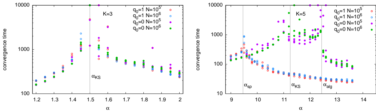
FIG. 11: Times to meet the BP convergence criterion (i.e. any marginal must change by less than 10^{-8} ) for k = 3 (left) and k = 5 (right), 2 system sizes ( N = 10^5, 10^6 ) and 2 different initial conditions ( q_0 = 0, 1 ). A data point with a time 10^4 means BP did not reach convergence.
