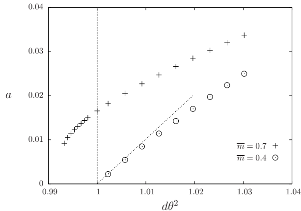
FIG. 7: The value of a in the fixed-point solution of the cavity equations reached from an informative initial condition, as a function of the signal-to-noise ratio, for the ferromagnetic ( \theta > 0 ) asymmetric Ising model. We used a regular degree distribution, \tilde{p}_\ell = \delta_{\ell,d} with d = 3 , each point correspond to a different value of \theta > 0 . The two set of symbols correspond to \bar{m} = 0.4 < \bar{m}_c and \bar{m} = 0.7 > \bar{m}_c . The vertical dashed line indicates the location of the Kesten-Stigum transition, while the inclined line is our analytical prediction from (116) for \bar{m} = 0.4 .
