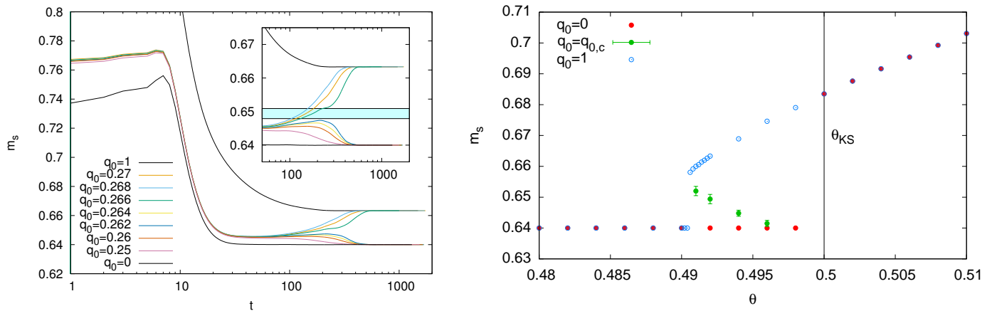
FIG. 17: The left panel illustrates the way we estimate the value of m_s for the unstable fixed point of BP (here \theta = 0.492 ), that plays the role of separatrix for the BP dynamics. The right panel reports these values obtained in the coexistence region \theta_{sp} < \theta < \theta_{KS} (here \bar{m} = 0.8 ).
