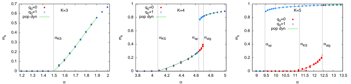
FIG. 10: The order parameter m_s detecting the planted configuration for k = 3 (left), k = 4 (center) and k = 5 (right), obtained by running BP on three samples of size N = 10^6 for each value \alpha . The lines are the predictions obtained by solving the cavity equations for the reconstruction problem on a tree, and plotted also in Fig. 6, with the correspondence m_s = 2a explained in the text.
