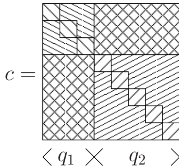
FIG. 5: The shape of the connectivity matrix in the q_1 + q_2 Potts model, matrix elements filled with the same pattern are equal.
