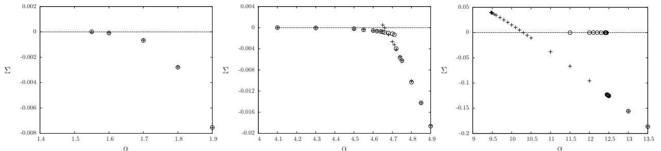
FIG. 9: The complexity \Sigma = -\phi for the fixed point solutions of the cavity equations for the hypergraph bicoloring problem, for k = 3, 4, 5 from left to right; the symbols are the same as in Fig. 6, crosses correspond to an informative initial condition, circles to an uninformative one.
