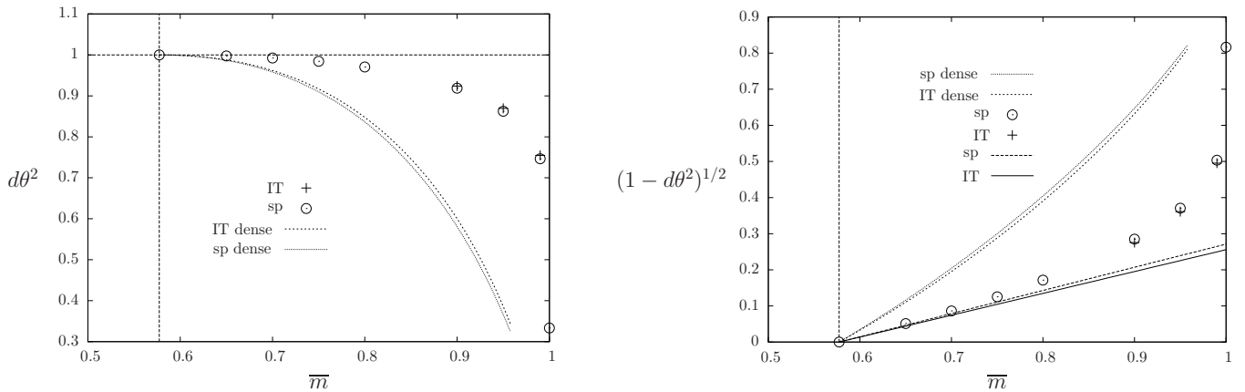
FIG. 4: The phase diagram of the ferromagnetic ( \theta > 0 ) asymmetric Ising model on a regular tree with offspring degree distribution \tilde{p}_\ell = \delta_{\ell,d} , d = 3 . The magnetization parameter \bar{m} encodes the size of the smaller tree community, in the SBM interpretation, as (1 - \bar{m})/2 . On the left panel the spinodal and IT transitions are plotted in terms of the signal-to-noise parameter d\theta^2 , which equals 1 at the Kesten-Stigum transition (horizontal dashed line). Within our numerical accuracy we cannot distinguish the spinodal and IT points for \bar{m} smaller than 0.8, we used a single symbol in this case. The two lines corresponds to the large degree limit, as computed for the dense models in [16, 26, 27]. On the right panel the same data is drawn in rescaled units to better appreciate the crossover from 1st to 2nd order transition as \bar{m} reaches its critical value \bar{m}_c = 1/\sqrt{3} \approx 0.577 , marked as a vertical line. The two straight lines are the analytical predictions of Eqs. (131,134) for the leading order behavior of the spinodal and IT transitions as \bar{m} \rightarrow \bar{m}_c^+ , for the sparse case \tilde{p}_\ell = \delta_{\ell,3} .
