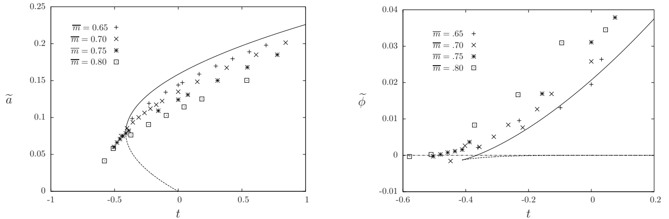
FIG. 8: Study of the scaling regime in the neighborhood of the point (\theta_{KS}, \bar{m}_c) for the ferromagnetic asymmetric Ising model with degree distribution \tilde{p}_\ell = \delta_{\ell,d} , d = 3 . The rescaled signal-to-noise ratio parameter is t = (d\theta^2 - 1)/(\bar{m} - \bar{m}_c)^2 , the Kesten-Stigum transition thus corresponds to t = 0 . Left panel: the rescaled accuracy \tilde{a} = a/(\bar{m} - \bar{m}_c) as a function of t ; the lines are the analytic predictions for the stable (solid) and unstable (dashed) branches of fixed-points obtained in Eq. (128), the symbols are numerical results that approach the analytic line when \bar{m} \rightarrow \bar{m}_c^+ . Right panel: the rescaled free-entropy \tilde{\phi} = \phi/(\bar{m} - \bar{m}_c)^4 as a function of t ; the analytic lines have been obtained by inserting in (132) the two branches of \tilde{a} from (128), the threshold t_{IT} corresponds to the crossing with the horizontal line \tilde{\phi} = 0 .
