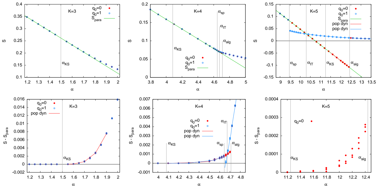
FIG. 13: Bethe RS entropy computed at the BP fixed points. The lower panels show the difference with respect to the paramagnetic entropy in order to show better the difference which is tiny in some cases. For k = 5 the difference is too small to be estimated reliably via population dynamics and so we report only data obtained via BP.
