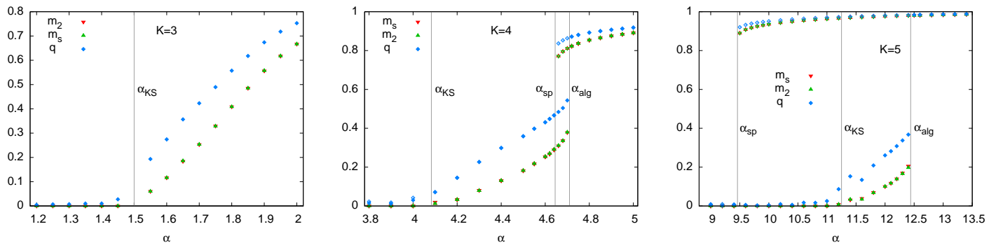
FIG. 12: Comparison between different order parameters detecting the planted configuration. Data have been averaged over the samples where BP reached a fixed point. As in Figure 10, filled (resp. empty) points correspond to q_0 = 0 (resp. q_0 = 1 ).
