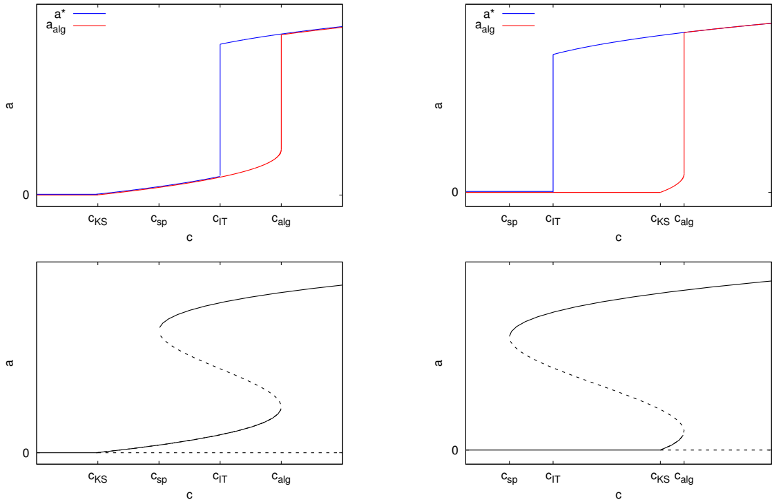
FIG. 2: Top: The “new” scenarios in terms of the Bayes-optimal ( a^* , in blue) and algorithmic ( a_{\text{alg}} , in red) performance. Bottom: The “new” scenarios in terms of the fixed points of eq. (6). Stable fixed points are in full line, unstable one are dashed. In all panels the accuracy a is plotted as a function of the signal-to-noise ratio c . The thresholds c_{\text{sp}} , c_{\text{IT}} , c_{\text{KS}} and c_{\text{alg}} , as defined in the text, are marked on the x-axes. The KS threshold c_{\text{KS}} here is strictly smaller than the algorithmic one c_{\text{alg}} . We note that the thresholds can also be ordered as c_{\text{sp}} < c_{\text{KS}} < c_{\text{IT}} < c_{\text{alg}} .
