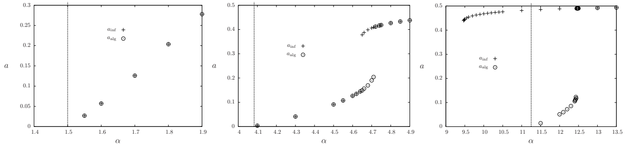
FIG. 6: Stable fixed points of the cavity equations in terms of their accuracies for the planted bicoloring of k -uniform hypergraphs, with k = 3, 4, 5 from left to right. The accuracy is defined here as the difference between the probability that a sample from the posterior marginal outputs the correct label and the same probability when only the prior is used, see Sec. IV K for more details. The vertical line marks the KS threshold. These curves have been obtained by a numerical resolution of the cavity equations (15,16), a_{\text{inf}} corresponds to the fixed point reached from an informative initialization (corresponding to the reconstruction problem, \varepsilon = 1 in Eq. (30)), a_{\text{alg}} was obtained from an uninformative initialization (corresponding to the robust reconstruction problem, \varepsilon \rightarrow 0 in Eq. (30)). The parameter \alpha controls the offspring degree distribution \tilde{p}_\ell , which is a Poisson law of average \alpha k . The optimal accuracy a^* coincides with a_{\text{inf}} above the IT transition, whose location can be found in Table I.
