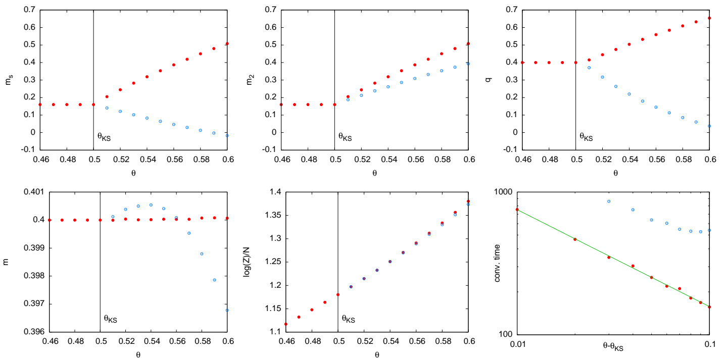
FIG. 16: Different fixed points reached by BP run with a non-informative initial condition on samples of the asymmetric SBM ( d = 4 , \bar{m} = 0.4 , N = 10^7 ). Red full points refer to the dominating fixed point having the largest \log(Z) , while blue empty points refer to the sub-dominating fixed point.
