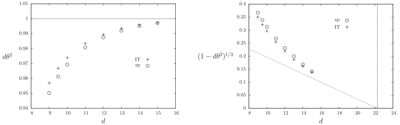
FIG. 3: The phase diagram of the 4 groups disassortative symmetric SBM (equivalently the reconstruction of antiferromagnetic q = 4 Potts model on Poissonian Galton-Watson trees), as a function of the average degree d . On the left panel the spinodal and IT transitions (see the text and Fig. 1 for their definitions) are plotted in terms of the signal-to-noise parameter d\theta^2 , which equals 1 at the Kesten-Stigum transition (horizontal dashed line). On the right panel the same data is drawn in rescaled units to better appreciate the crossover from 1st to 2nd order transition as d increases; the vertical line marks our analytical prediction for d_c \approx 22.2694 , the other line is only here as a guide to the eye.
