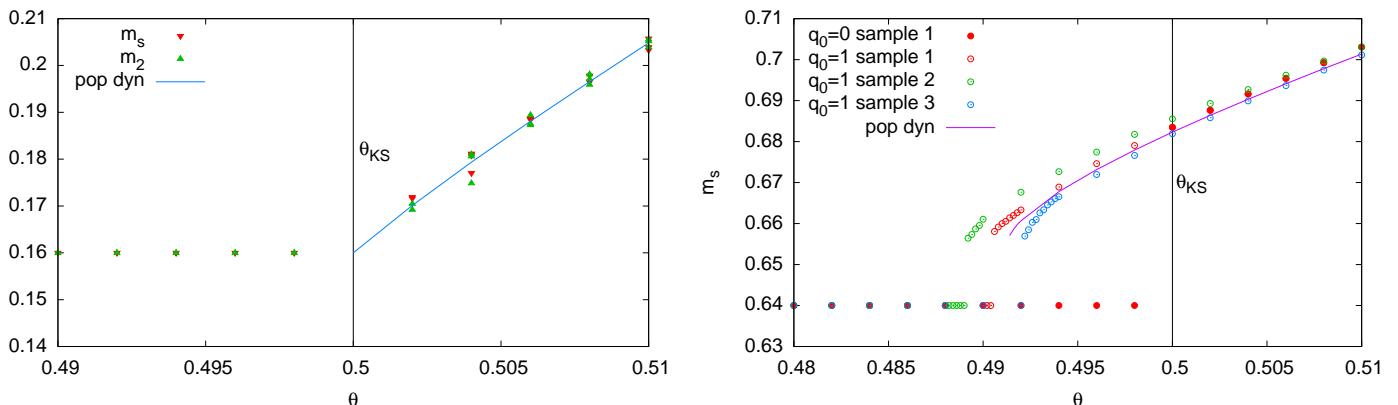
FIG. 15: Comparison between BP and population dynamics in detecting the planted configuration in the asymmetric SBM with d = 4 . For each \theta value we have simulated 3 samples of size N = 10^7 . The asymmetry is \bar{m} = 0.4 < \bar{m}_c in the left panel and \bar{m} = 0.8 > \bar{m}_c in the right panel. In both cases the planted configuration can be detected purely from the graph ( q_0 = 0 ) for \theta > \theta_{KS} . Despite visible sample-to-sample fluctuations the prediction by population dynamics is always very faithful.
