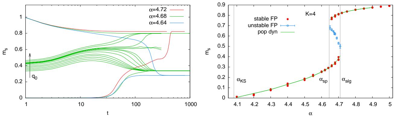
FIG. 14: Search for the unstable fixed point of BP in the range [\alpha_{sp}, \alpha_{alg}] . In the left panel, lowermost (resp. uppermost) curves have been obtained with q_0 = 0 (resp. q_0 = 1 ); the rest of the curves for \alpha = 4.68 have been obtained varying q_0 by \Delta q_0 = 0.01 in the range [0.2, 0.29] and by \Delta q_0 = 0.002 in the range [0.26, 0.27] .
