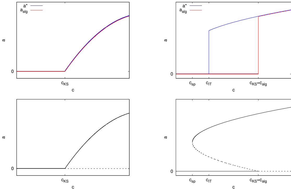
FIG. 1: Top: The “standard” scenarios in terms of the Bayes-optimal ( a^* , in blue) and algorithmic ( a_{\text{alg}} , in red) performance. Bottom: The “standard” scenarios in terms of the fixed points of eq. (6). Stable fixed points are in full line, unstable ones are dashed. In all panels the accuracy a is plotted as a function of the signal-to-noise ratio c . The thresholds c_{\text{sp}} , c_{\text{IT}} , c_{\text{KS}} and c_{\text{alg}} , as defined in the text, are marked on the horizontal axes.
