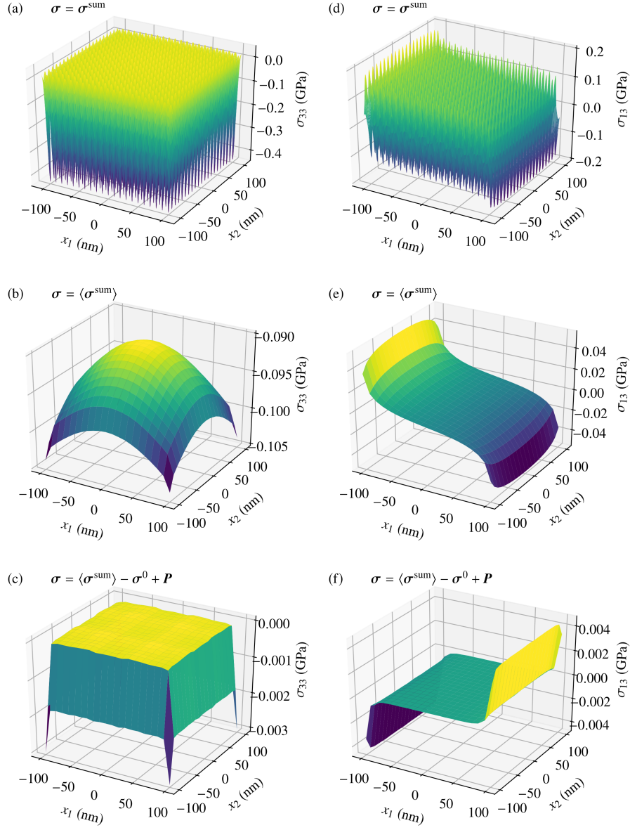
Figure 3: Stresses \sigma_{33} (a-c) and \sigma_{13} (d-f) on a surface of normal [001] of a macroscopic system containing 21 \times 21 \times 21 simulation boxes: (a,d) stress \sigma = \sigma^{\text{sum}} due to the contribution of defects inside the system (b,e) average stress \sigma = \langle \sigma^{\text{sum}} \rangle over the simulation box dimensions (c,f) average stress corrected by the non-periodic part \sigma^0 and the dipole density: \sigma = \langle \sigma^{\text{sum}} \rangle - \sigma^0 + P . The simulation box contains one prismatic loop (see text for details).
