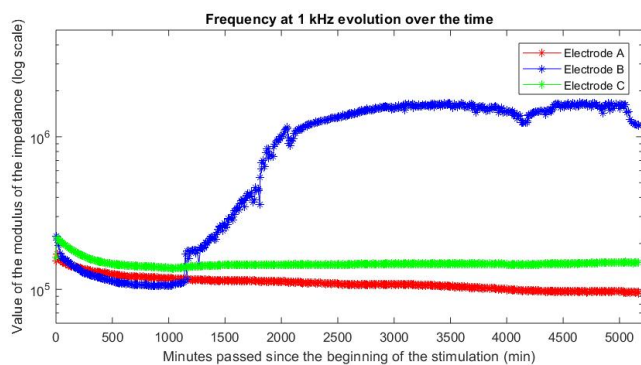
Fig. 4. Evolution of the impedance module at 1 kHz for a strip of 60 um diamond microelectrodes.
