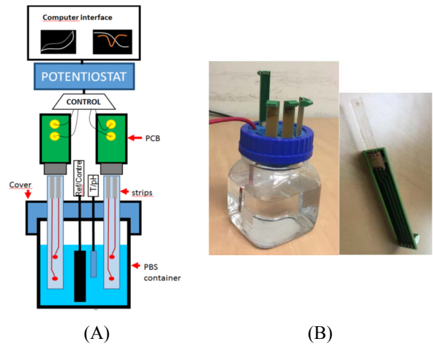
Fig. 2. Configuration of the ageing modular system (A) and example of strips used (B)
