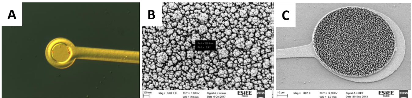
Fig. 1. Optical and SEM images of fabricated microelectrodes: gold (a), black platinum (b) and diamond (c)
