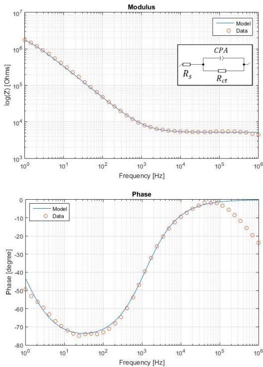
Fig. 3. Fitting of the EIS measured data from a 60 um diameter black platinum electrode to the described model
