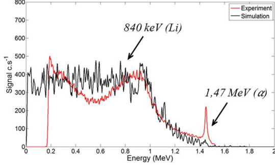
Fig. 4. Experimental and simulated spectra obtained with CPNB48.
