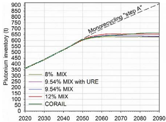
Fig. 12. Plutonium inventory.
