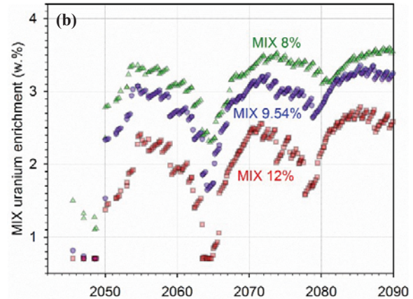
Fig. 7. Pu content in MOX rods of fresh CORAIL assemblies (a) and uranium enrichment in new MIX fuels (b).
