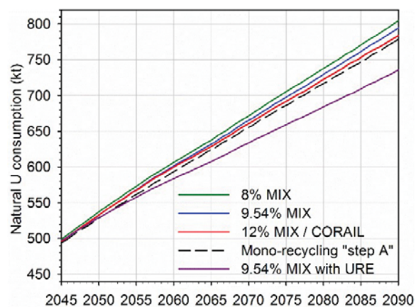
Fig. 5. Natural uranium consumption.
