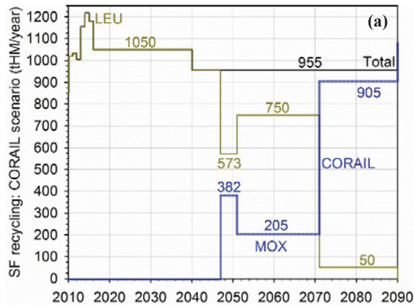
Fig. 9. Fuel reprocessing during the CORAIL scenario (a) and during the 9.54% MIX scenarios (b).
