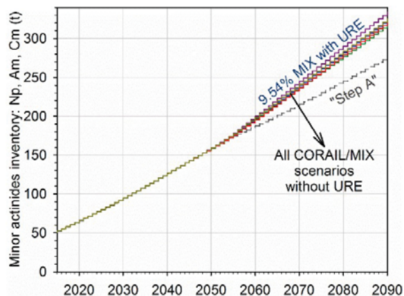
Fig. 13. Minor actinides.
