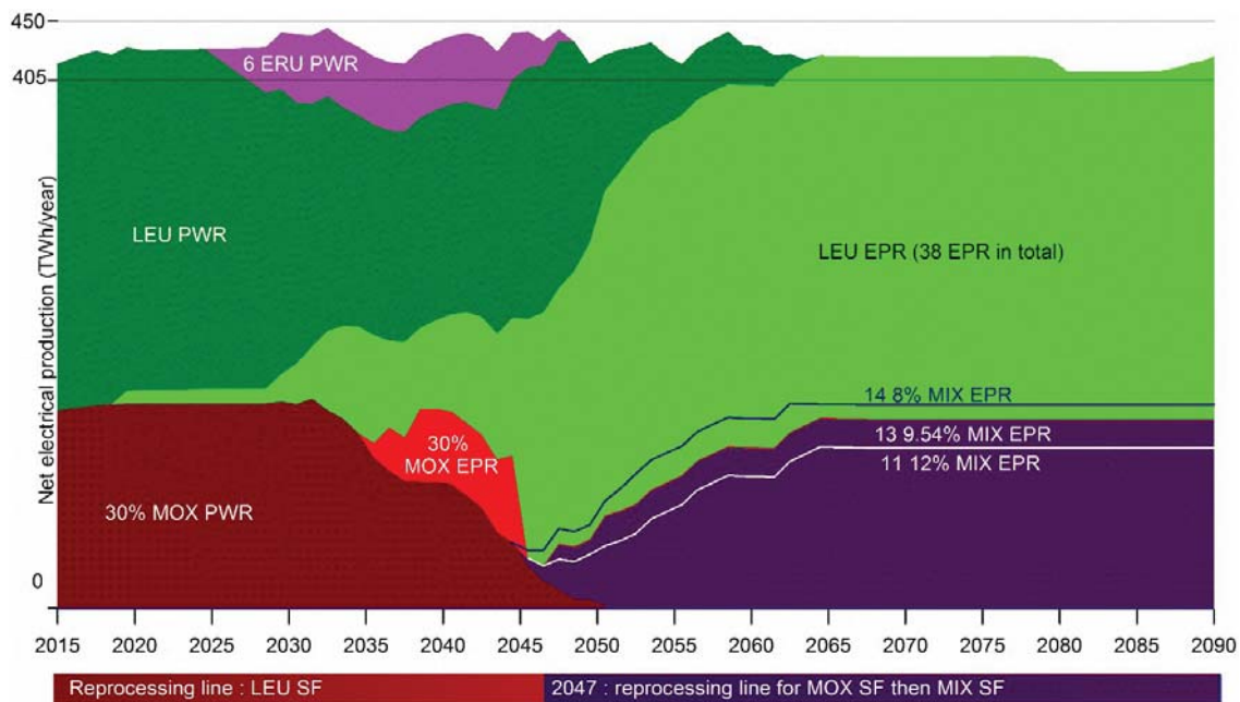
Fig. 3. Scenarios MIX without uranium recycling into ERU fuel.
