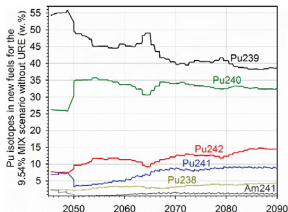
Fig. 6. Plutonium isotopic composition of MIX new fuels for the 9.54% MIX scenario.
