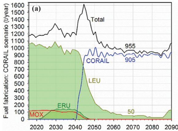
Fig. 8. Fuel fabrication during the CORAIL scenario (a) and during the 9.54% MIX with ERU scenario (b).
