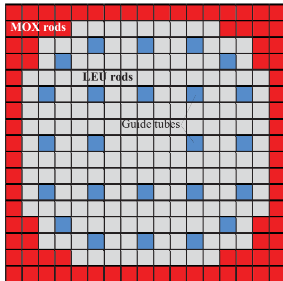
Fig. 1. CORAIL 17×17 heterogeneous assembly in EPR.
