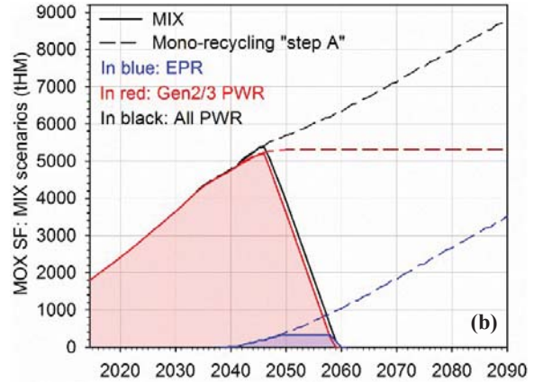
Fig. 10. MOX spent fuels for the CORAIL (a) and MIX (b) scenarios.
