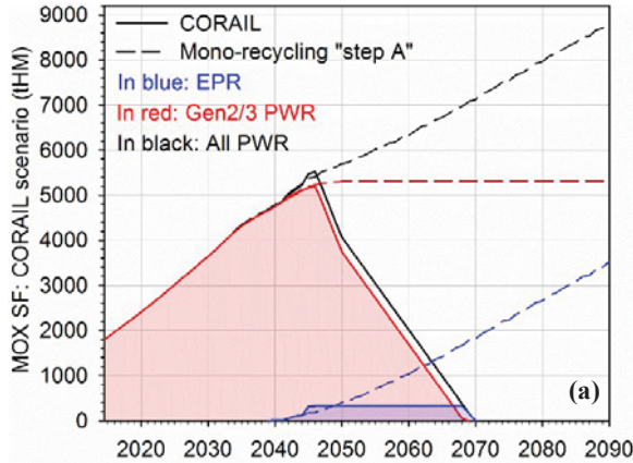
Fig. 10. MOX spent fuels for the CORAIL (a) and MIX (b) scenarios.
