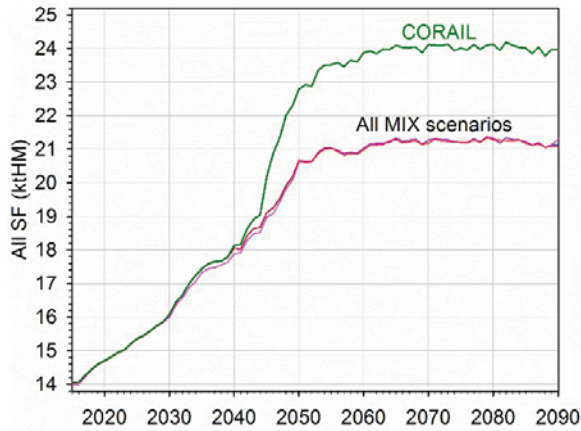
Fig. 11. Spent fuels: total quantity.
