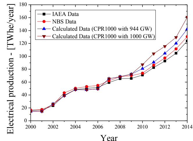
Fig. 8. Electricity production up to 2014.
