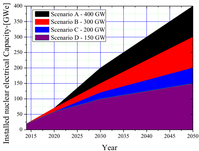
Fig. 4. Various evolutions of the nuclear power up to 2050.
