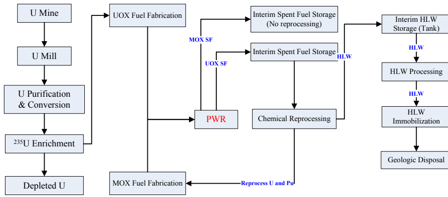
Fig. 6. “Pu recycled in PWR”.
