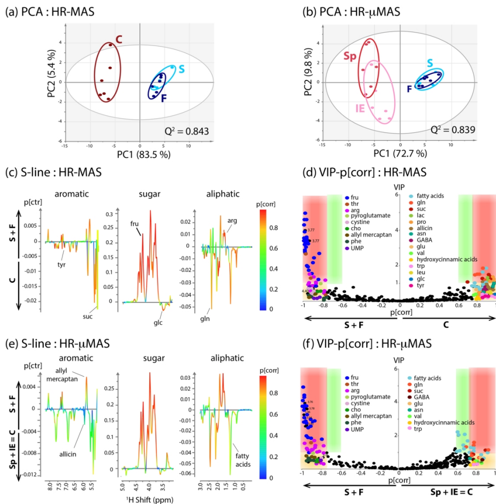
Figure 3 PCA score plots obtained for the separation of the garlic regions using the (a) HR-MAS spectral data and (b) HR- \mu MAS. The spectra data corresponding to skin (S), flesh (F) and core (C) for HR-MAS; and S, F, sprout (Sp) and inner epidermis (IE) for HR- \mu MAS, are clustered in specific colors for a better readability. Quality parameters: for HR-MAS, 3-components, R2X = 0.919 , Q2 = 0.843 ; for HR- \mu MAS, 5-components, R2X = 0.934 , Q2 = 0.839 . The corresponding OPLS-DA were carried out to identify the latent variants. The S-line plots (c) HR-MAS and (e) HR- \mu MAS identify a few significant variables in S+F ( p[ctr] > 0 ) and C ( p[ctr] < 0 ) in HR-MAS, or Sp+IE ( p[ctr] < 0 ) in HR- \mu MAS. The significant level p[corr] is indicated by a color scheme. The VIP-p[corr] plots (d) HR-MAS and (f) HR- \mu MAS facilitate the identification of a complete list of metabolic variants. Quality parameters of OPLS-DA: for HR-MAS, 1 predictive component and 1 orthogonal component, R2X = 0.888 , R2Y = 0.982 , Q2 = 0.968 , p-value (CV) = 7.61 \cdot 10^{-9} ; and for HR- \mu MAS, 1 predictive component and 1 orthogonal component, R2X = 0.806 , R2Y = 0.975 , Q2 = 0.964 , p-value (CV) = 1.81 \cdot 10^{-13} .
