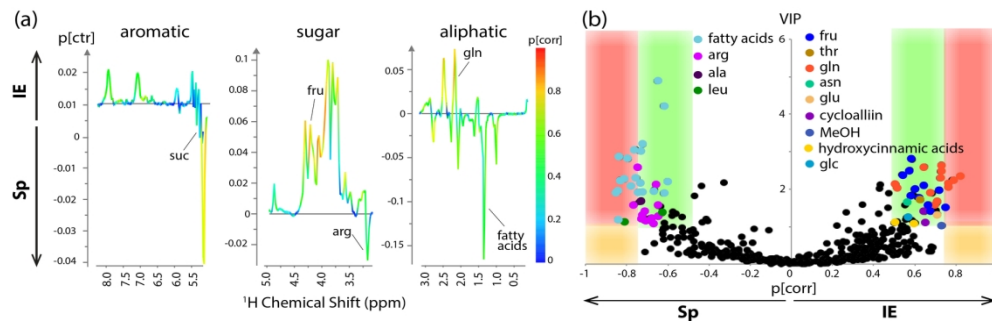
Figure 4 (a) S-line plot and (b) VIP- p[\text{corr}] plot used to identify the significant variables responsible of variations between Sp and IE. Quality parameters of OPLS-DA: 1 predictive component and 2 orthogonal components, R2X = 0.747 , R2Y = 0.955 , Q2 = 0.828 , p\text{-value (CV)} = 0.027 .
