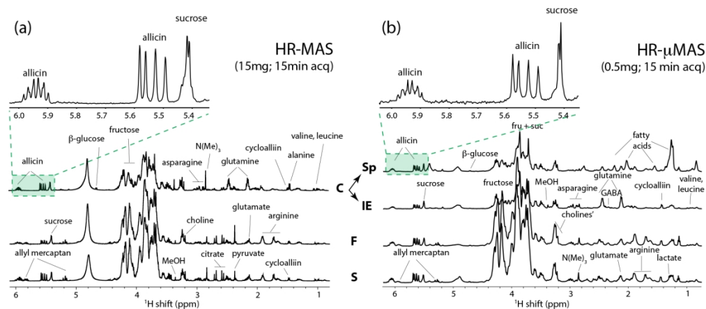
Figure 2 Spectral comparison of the garlic regions between (a) HR-MAS and (b) HR- \mu MAS. The intensities are normalized to that of the sucrose signal at 5.42 ppm. The assigned metabolites are indicated. The chemical shift range between 5.3–6.0 ppm is amplified showcasing the spectral quality.
