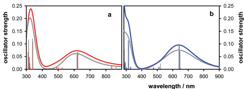
Fig. 5 Absorption spectra computed for the (AT) 1 •+ radical cation ((a), red) and the [(AT) 1 -6H] • deprotonated radical ((b), blue). The corresponding spectra of 9-methyl-adenine are shown in grey. The sticks represent individual electronic transitions. Calculated at the PCM/TD-M052X/6-31G(d)//M052X/6-31G(d) level of theory.
