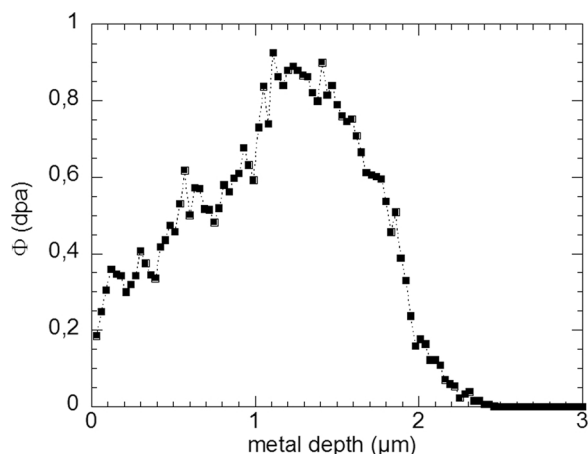
Fig. 2. SRIM simulation of nuclear damage in the metal after 6 MeV Zr ion irradiation at a fluence of 4 \times 10^{14} \text{ cm}^{-2} (calculations in Full Cascade mode).
