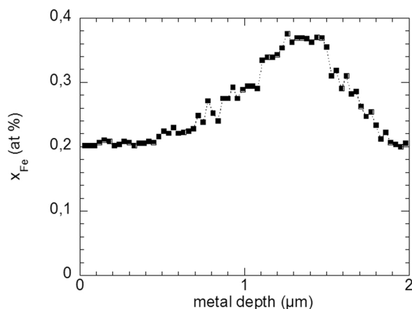
Fig. 3. SRIM simulation of iron implantation in the metal after 1 MeV iron ion irradiation at a fluence of 5 \times 10^{15} \text{ cm}^{-2} (calculations in Full Cascade mode).
