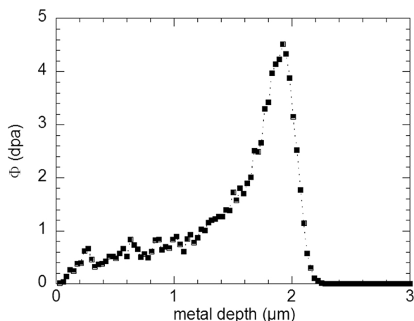
Fig. 1. SRIM simulation of nuclear damage in the metal after 300 keV proton irradiation at a fluence of 10^{18} \text{ cm}^{-2} (calculations in Full Cascade mode).
