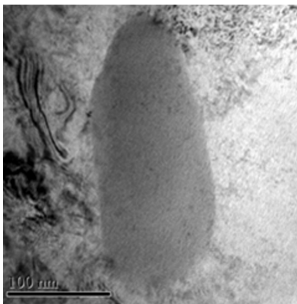
Fig. 6. Bright field TEM image of the matrix irradiated with Fe ions at a fluence of 2.5 \times 10^{15} and 5 \times 10^{15} \text{ cm}^{-2} and an amorphous precipitate \text{Zr(Fe,Cr)}_2 (no contrast inside the SPP).
