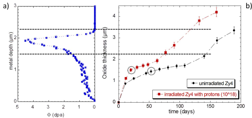
Fig. 7. a) Damage profile in the matrix of Zy4 sample irradiated with 300 keV protons at a fluence of 10^{18} \text{ cm}^{-2} and 350 °C. b) Oxidation kinetics of unirradiated sample and sample irradiated with 300 keV protons at a fluence of 10^{18} \text{ cm}^{-2} and 350 °C. Black dotted circles indicate the oxide thicknesses at which the samples were exposed in ^{18}\text{O} enriched environment.
