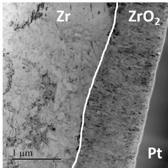
Fig. 12. Cross-section TEM image of the oxide layer formed on the proton irradiated metal during 14 days exposure time.
