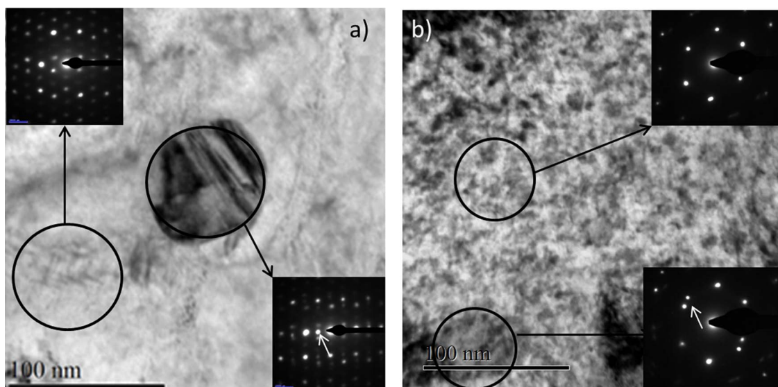
Fig. 4. a) Bright field TEM image and electron diffraction patterns of the unirradiated matrix and a crystalline precipitate \text{Zr(Fe,Cr)}_2 (the white arrow indicates a dot corresponding to the diffraction of the crystalline precipitate). b) Bright field TEM image and electron diffraction patterns of the irradiated matrix with 300 keV protons at a fluence of 10^{18} \text{ cm}^{-2} and a crystalline precipitate \text{Zr(Fe,Cr)}_2 (the white arrow indicates a dot corresponding to the diffraction of the crystalline precipitate).
