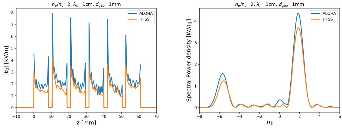
Figure 2: Example of comparison between ALOHA and HFSS ( n_e = 2n_c , \lambda_n = 1 cm, 1 mm vacuum gap). Left: toroidal component of the electric field at the mouth of the antenna. Right: Power density spectrum excited by the antenna.
