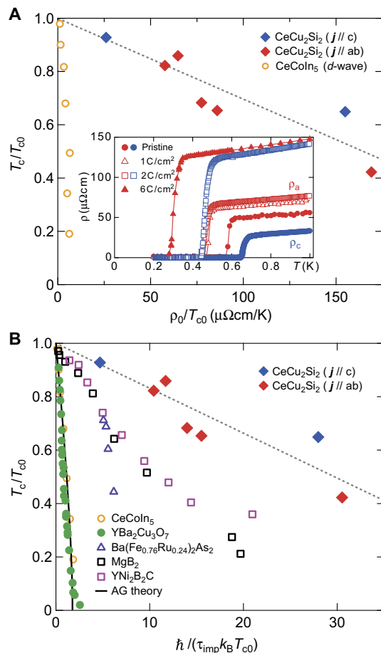
Fig. 5. Pair-breaking effect of CeCu 2 Si 2 . (A) Suppression of superconducting transition temperature T_c/T_{c0} as a function of \rho_0/T_{c0} , which is proportional to the pair-breaking parameter for CeCu 2 Si 2 and Sn-substituted CeColn 5 (d-wave) (30). Here, T_{c0} is the transition temperature with no pair-breaking effect and \rho_0 is the residual resistivity. For CeCu 2 Si 2 , T_{c0} = 0.71 K is used. Inset shows the temperature dependence of resistivity in CeCu 2 Si 2 before and after electron irradiation, which creates point defects. (B) Comparison of impurity effect of CeCu 2 Si 2 with those of other superconductors. Suppression of superconducting transition temperature T_c/T_{c0} as a function of dimensionless pair-breaking parameter \hbar/(\tau_{\text{imp}}k_B T_{c0}) . The solid line shows the prediction of the Abrikosov-Gor'kov (AG) theory for an isotropic s-wave superconductor with magnetic impurities. We also plot the data for Sn-substituted CeColn 5 (d-wave) (30), electron-irradiated YBa 2 Cu 3 O 7- \delta (31), electron-irradiated Ba(Fe 0.76 Ru 0.24 ) 2 As 2 (possibly s_{\pm} wave) (32), and neutron-irradiated MgB 2 (33) and YNi 2 B 2 C (35). The value of T_{c0} is estimated by extrapolating two initial data points to zero 1/\tau_{\text{imp}} limit. Rather weak pair-breaking effect in Ba(Fe 0.76 Ru 0.24 ) 2 As 2 has been attributed to a large imbalance between intra- and interband scattering (32). For MgB 2 data, we use the value of \lambda_{ab}(0) = \lambda_c(0) = 100 nm (34). For YNi 2 B 2 C data, we use \lambda_{ab}(0) = 110 nm (36) and \lambda_c(0) = \lambda_{ab}(0)H_{c2}^{ab}/H_{c2}^c = 140 nm (37), where H_{c2}^{ab} and H_{c2}^c are upper critical fields parallel and perpendicular to the ab plane.
