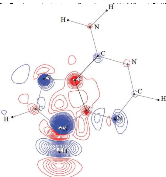
Fig. 5 Difference contour plots of electronic densities between neutral 9A( X^1A' ) and its cation 9A+( X^2A^0 ), where both species are taken at the equilibrium geometry of the neutral. The blue (red) lines correspond to regions where the density in 9A is higher (lower) than in 9A+. We plot the first contour for 0.02 \text{ e Bohr}^{-3} . The step between the contours is 0.02 \text{ e Bohr}^{-3} . These computations are done at the CASSCF/aug-cc-pVDZ level and drawn using the MOLDEN package. 75
