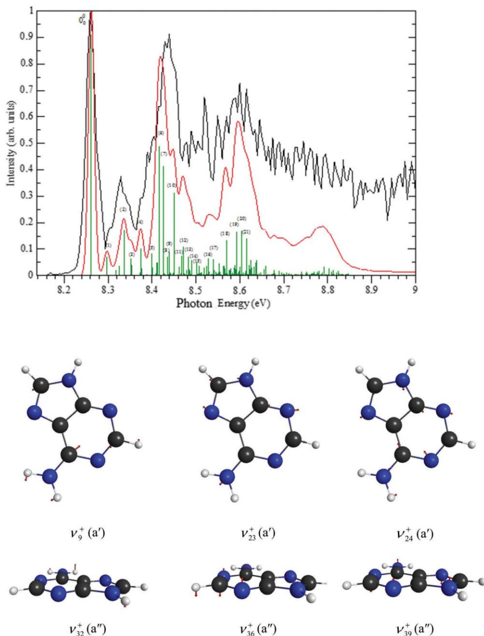
Fig. 4 Upper trace: Simulated (red line) and SPES of 9A (black line) in the 8.1–9 eV range. The tentative assignment of these peaks is given in Table S2 of the ESI.† Lower trace: Normal modes of 9A used for the assignment. The computed intensities are renormalized to that of the Q^0 transition.
