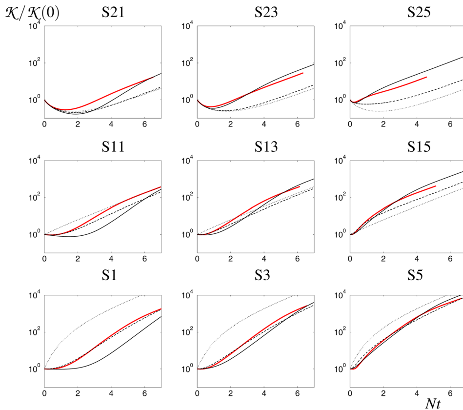
Fig. 9 Evolution of the kinetic energy \mathcal{K} as a function of time Nt for different cases S^* with Saffman initial spectra. (Thick red plain line) EDQNM, (thin plain line) 2SFK, (dashed line) GSG+, and (dotted line) \mathcal{K} - \mathcal{E} .
