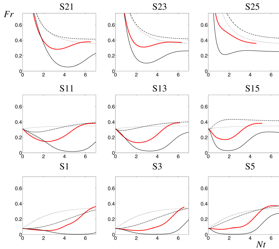
Fig. 10 Evolution of the Froude number Fr = \varepsilon/\kappa N as a function of time Nt for different cases S^* with Saffman initial spectra. (Thick red plain line) EDQNM, (thin plain line) 2SFK, (dashed line) GSG+, and (dotted line) \kappa-\varepsilon .
