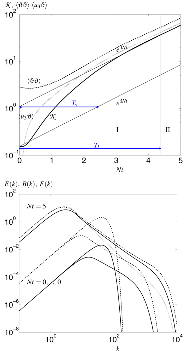
Fig. 3 (Top) Time-evolution of the kinetic energy \mathcal{K} (plain curve), the variance of buoyancy \langle \vartheta \vartheta \rangle (dashed curve) and the vertical buoyancy flux \langle u_3 \vartheta \rangle (dotted curve) corresponding to run S15. (Bottom): Energy spectrum E(k) (plain curve), buoyancy spectrum B(k) (dashed curve), and vertical velocity-buoyancy spectrum F(k) (dotted curve) as a function of wave-number k for run S15. Different times are shown corresponding to the initialization at Nt < 0 , when stratification effects are applied Nt = 0 and during self-similar regime Nt = 5 . F(k) is non-zero only for t > 0 .
