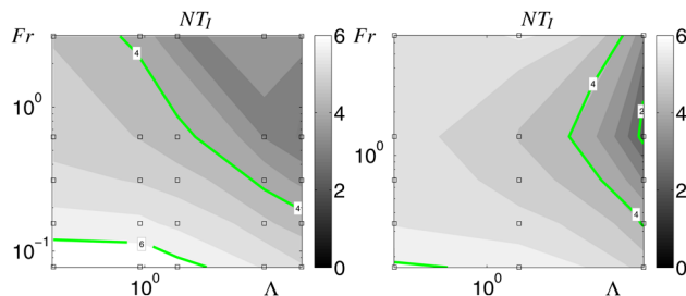
Fig. 4 Nondimensional transition delay NT_I as a function of initial Froude and mixing parameter and obtained from Eq. (2) for the k^2 Saffman spectra. The square symbols correspond to the simulations points of Table 1.
