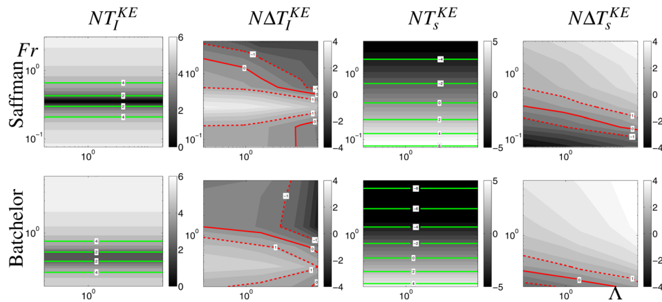
Fig. 6 Transition delays T_I^{KE} and time shifts T_s^{KE} as a function of the initial mixing parameter \Lambda (abscissa) and the Froude number Fr (ordinate) obtained from Eqs. (2) and (3) for the \mathcal{K} - \mathcal{E} model. Also, the differences between EDQNM and the \mathcal{K} - \mathcal{E} model on transition delays \Delta T_I^{KE} = T_I - T_I^{KE} and on time shifts \Delta T_s^{KE} = T_s - T_s^{KE} are represented. Cases for Saffman (top) and Batchelor (bottom) initial spectra are represented.
