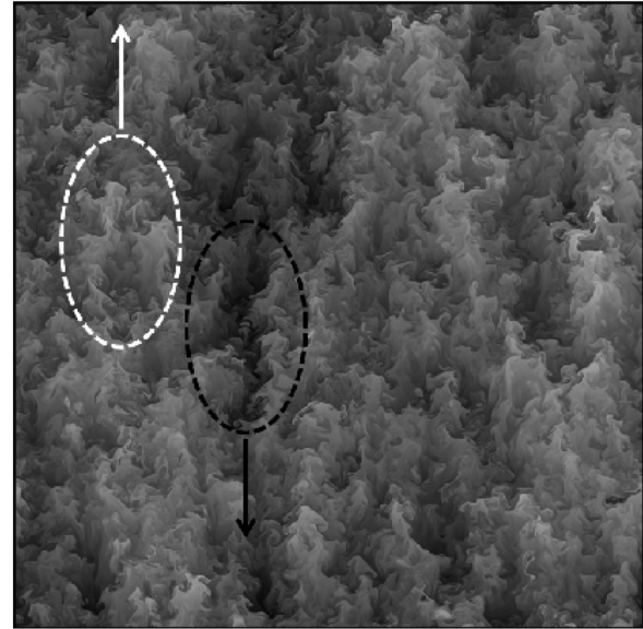
Fig. 1 Visualization of the buoyancy parameter \vartheta in a vertical plane of an USHT DNS. The acceleration points to the bottom in the figure. White zones, corresponding to lighter fluid, move upward while heavier darker parcels of fluid move downward.
