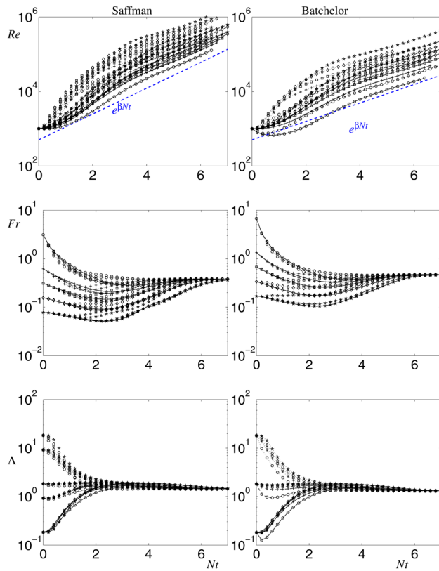
Fig. 2 Evolution of nondimensional numbers as a function of time for the different EDQNM simulations corresponding to Table 1; (top) Reynolds number, (middle) Froude number, (bottom) mixing parameter. (Left) Saffman k^2 spectra with symbols corresponding to initial Froude number; (circle) Fr = 3.1 , (cross) Fr = 0.62 , (square) Fr = 31 , (diamond) Fr = 0.155 , and (star) Fr = 0.078 . Lines correspond to the initial mixing parameter; (plain) \Lambda = 0.184 , (dashed) \Lambda = 0.92 , (dashed-dotted) \Lambda = 1.84 , (dotted) \Lambda = 9.2 , and (none) \Lambda = 18.4 . (right) Batchelor k^4 spectra with symbols corresponding to initial Froude number; (circle) Fr = 6.61 , (cross) Fr = 1.28 , (square) Fr = 0.67 , (diamond) Fr = 0.337 , and (star) Fr = 0.168 . Lines correspond to initial mixing parameter; (plain) \Lambda = 18.1 , (dashed) \Lambda = 1.81 , (dashed-dotted) \Lambda = 0.184 , and (dotted) \Lambda = 9.2 .
