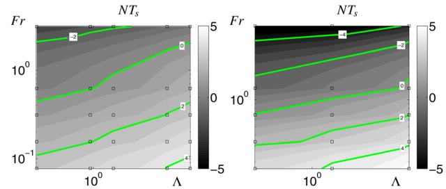
Fig. 5 Nondimensional time shift NT_s as a function of initial Froude and mixing parameter and obtained from Eq. (2) for the k^4 Batchelor spectra. The square symbols correspond to the simulations points of Table 1.
