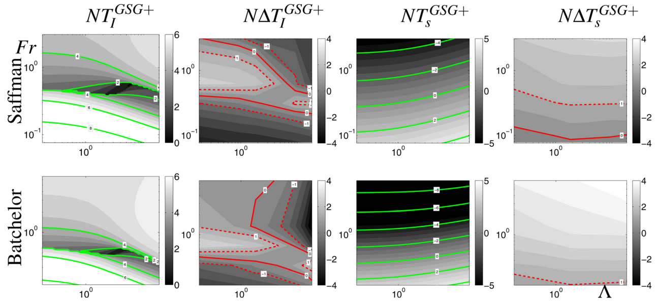
Fig. 7 Transition delays T_I^{GSG+} and time shifts T_s^{GSG+} as a function of the initial mixing parameter \Lambda (abscissa) and the Froude number Fr (ordinate) obtained from Eqs. (2) and (3) for the RSM GSG+ model. Also, the differences between EDQNM and the GSG+ model on transition delays \Delta T_I^{GSG+} = T_I - T_I^{GSG+} and on time shifts \Delta T_s^{GSG+} = T_s - T_s^{GSG+} are represented. Cases for Saffman (top) and Batchelor (bottom) initial spectra are represented.
