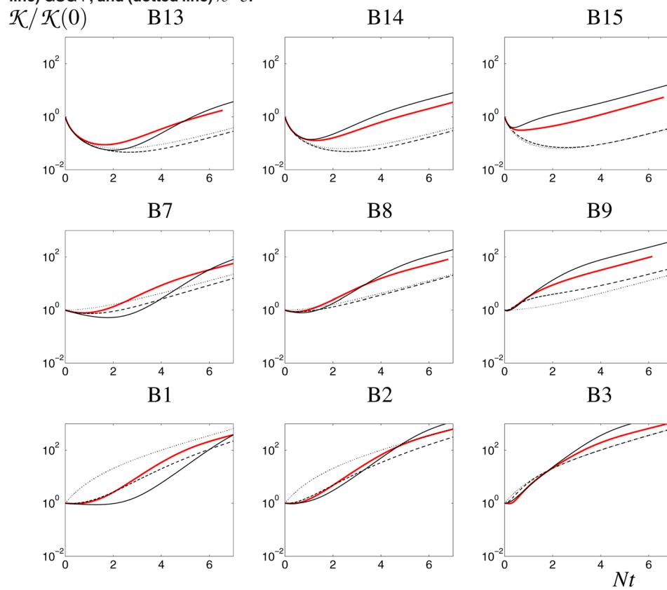
Fig. 11 Evolution of the kinetic energy \kappa as a function of time Nt for different cases B^* with Batchelor initial spectra. (Thick red plain line) EDQNM, (thin plain line) 2SFK, (dashed line) GSG+, and (dotted line) \kappa-\varepsilon .
