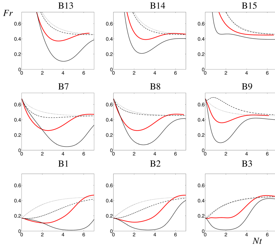
Fig. 12 Evolution of the Froude number Fr = \varepsilon/\kappa N as a function of time Nt for different cases B^* with Batchelor initial spectra. (Thick red plain line) EDQNM, (thin plain line) 2SFK, (dashed line) GSG+, and (dotted line) \kappa - \varepsilon .
