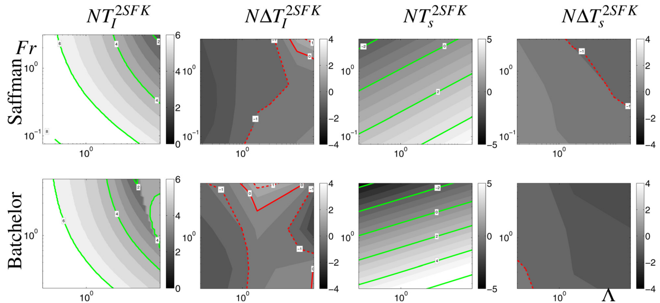
Fig. 8 Transition delays T_I^{2SFK} and time shifts T_s^{2SFK} as a function of the initial mixing parameter \Lambda (abscissa) and the Froude number Fr (ordinate) obtained from Eqs. (2) and (3) for the 2SFK model. Also, the differences between EDQNM and the 2SFK model on transition delays \Delta T_I^{2SFK} = T_I - T_I^{2SFK} and on time shifts \Delta T_s^{2SFK} = T_s - T_s^{2SFK} are represented. Cases for Saffman (top) and Batchelor (bottom) initial spectra are represented.
