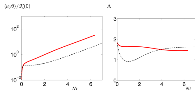
Fig. 13 (Left) Evolution of the vertical buoyancy flux \langle u_3 \delta \rangle / \kappa(0) , (right) evolution of the mixing parameter \Lambda as a function of time Nt for the S23 case. (Thick red plain line) EDQNM and (dashed line) GSG+.
