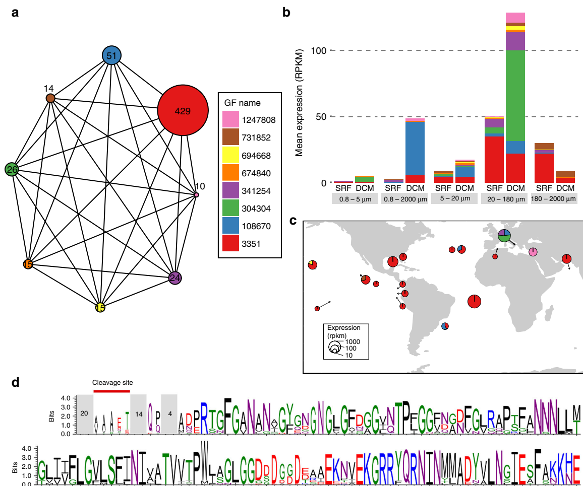
Fig. 5 New gene families expressed in 20–180 μm size fraction. a Graph representation of the protein group number 14079. Each GF of the protein group is represented by a node with a diameter proportional to the number of unigenes in the GF. Protein matches between GFs are represented by an edge. b Mean expression of GFs in different size-fractions and depths. Each color corresponds to a GF of protein group 14079. c World map representation of protein group 14079 expression in the 20–180 μm size fraction. SRF and DCM samples have been pooled. Circle diameters represent the relative expression of the protein group in RPKM. The contribution to expression of each GF is represented by the different colors. d Sequence logo of the multiple alignments of the protein group 14079. 45 ORFs (153 amino acids in average) of protein group 14079 were aligned and positions with more than 50% of gaps were removed. Mean numbers of amino acids on unaligned regions of the protein are indicated in gray boxes. A signal peptide cleavage site, indicated on the left part of the sequence logo was predicted on 21 sequences
