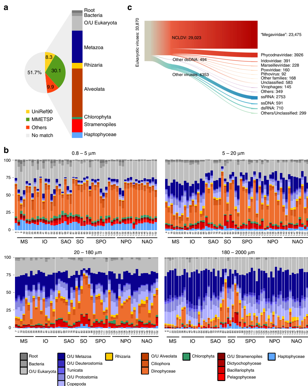
Fig. 2 Taxonomic composition of the gene catalog. a Origin of the best similarity sequence match as a fraction of the total in the circular diagram (MMETSP 14 ; release of August 2014, with manual curation; UniRef90 42 ; release of September 2014; “Others”: are other reference transcriptomes that were added as reference to offset the lack of knowledge about organisms in large size fractions, in particular copepods and rhizaria; Methods section). Unigenes without significant matches (i.e., those with an e -value >10^{-5} for their best similarity match) are tagged as “No match”. The proportion of unigenes affiliated to each major taxonomic group is indicated in the right column. O/U, other or unassigned. b Proportion of each major taxonomic group across Tara Oceans stations based on the mean number of unigenes classified as one of 24 different single-copy ribosomal proteins detected in each sample (IO, Indian Ocean; MS, Mediterranean Sea; NAO, North Atlantic Ocean; NPO, North Pacific Ocean; SAO, South Atlantic Ocean; SO, Southern Ocean; SPO, South Pacific Ocean). c Eukaryotic viral unigenes. NCLDV unigenes are classified at the family level
