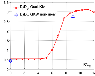
Figure 6. Ratio of ion to electron particle diffusivities versus R/L_{T_i} (other parameters from GA standard case, see Table 1). The red circles are for QuaLiKiz ratios and the blue stars for GKW ratios as given in Table 2.
