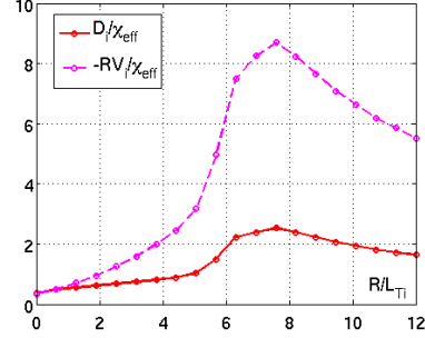
Figure 9. Ratio of the ion diffusivity and convective terms to \chi_{eff} , versus R/L_{Ti} (other parameters from GA standard case, see Table 1).
