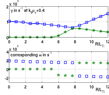
Figure 5. Upper figure: growth rate at k_\theta \rho_s = 0.4 for the two most unstable branches versus R/L_{T_i} (other parameters from GA standard case, see Table 1). Lower figure: corresponding frequency versus R/L_{T_i} , when negative (resp. positive) the mode drifts in the ion (resp. electron) diamagnetic direction. Blue squares stand for the most unstable branch, green stars for the subdominant branch.
