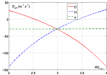
Figure 15. Effective diffusion in m^2.s^{-1} plotted with respect to R/L_{nH} . In full line, red, for D, in dashed blue line for H and in green dash-dotted line, for electrons.
