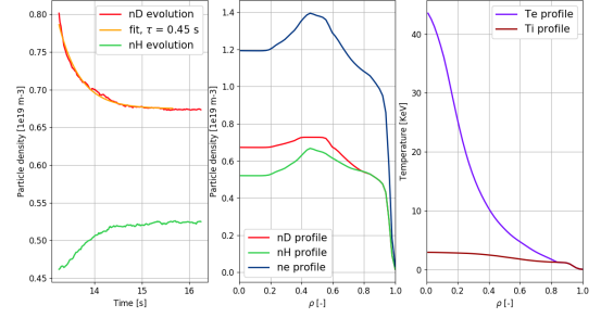
Figure 21. TEM dominated regime. Evolution of D and H density at \rho = 0.6 when turning off the particle source (left panel). Relaxed density (central panel) and temperature (right panel) profiles at 16 s.
