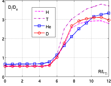
Figure 11. Ratio of ion to electron diffusivities, versus R/L_{Ti} for H, D, T and He without collisions (other parameters from GA standard case, see Table 1). Magenta dashed line and smaller circles: H. Red line and circles: D. Darker red dot-dashed line and smaller circles: T. Blue line and squares: He.
