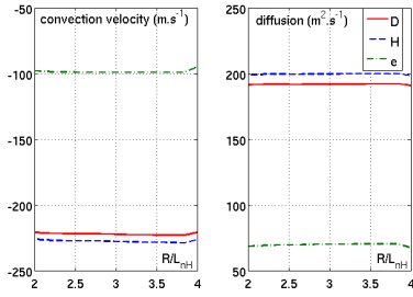
Figure 14. Convection velocity in m.s^{-1} and diffusion coefficient in m^2.s^{-1} are plotted with respect to R/L_{nH} . In full line, red, for D, in dashed blue line for H and in green dash-dotted line, for electrons.
