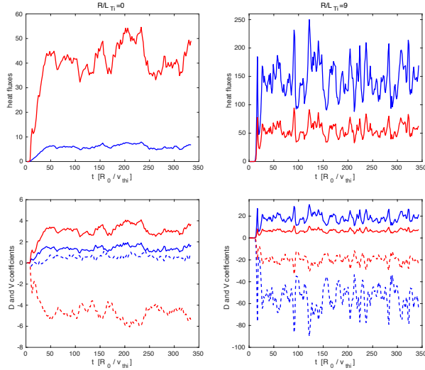
Figure 1. Top row: time evolution of the electron (red) and ion (blue) heat fluxes in the non-linear simulations at R/L_{T_i} = 0 (left column) and R/L_{T_i} = 9 (right column). Bottom row: corresponding particle diffusivity (full lines, D_e in red and D_i in blue) and particle pinch (dashed lines, V_e in red and V_i in blue). The heat fluxes are normalised to nT\rho_*^2 v_{\text{thi}} , the diffusivities to \rho_*^2 v_{\text{thi}} R and the pinch coefficients to \rho_*^2 v_{\text{thi}} .
