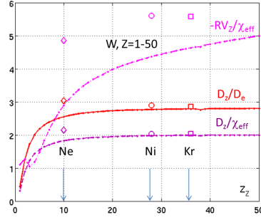
Figure 12. Ratio between the trace impurity diffusivity and 1/ the electron diffusivity (red) 2/ the effective heat diffusivity (purple), ratio between the trace impurity convective velocity (magenta) and the effective heat diffusivity versus Z_Z , for the ITG1 case (see Table 1). For A_Z = 184 , corresponding to W, with a charge Z_Z varying from 1 to 50 (full lines), for Ne A_Z = 20 and Z_Z = 10 (diamonds), for Ni A_Z = 56 and Z_Z = 28 (circles) and for Kr A_Z = 78 and Z_Z = 36 (squares).
