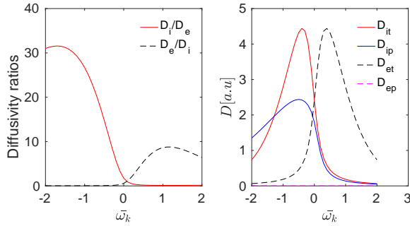
Figure 2. Ratios of D_i/D_e and D_e/D_i for a range of input frequencies (left panel), corresponding to a direct calculation of Eq. 9, with \bar{\gamma} = 0.2 . The right panel shows the breakdown of the contribution to the diffusivities according to trapped and passing ions, and trapped and passing electrons. Note that the passing electron contribution is always negligible.
