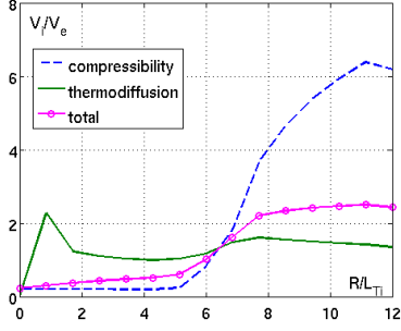
Figure 7. Ratio of ion to electron convective velocities, versus R/L_{Ti} (other parameters from GA standard case, see Table 1). Magenta circles: ratio of the total convective velocities. Blue dashed lines: ratio of the compressibility components. Green full lines: ratio of the thermodiffusion components.
