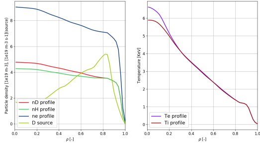
Figure 16. Relaxed density profiles for a D particle source (left panel) and ion and electron temperature profiles (right panel), for n_H = n_D at \rho = 0.85 , at 13 s.
