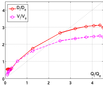
Figure 8. Ratio of ion to electron diffusivities and convective velocities versus Q_i/Q_e (other parameters from GA standard case, see Table 1). Magenta dashed line circles: ratio of the total convective velocities. Red line and circles: ratio of the diffusivities.
