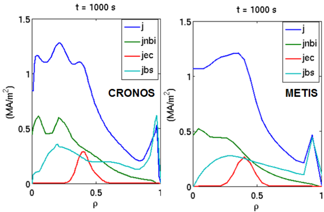
Figure 13: ITER hybrid scenario: computed current density profile and contributions from NBI, ECCD and bootstrap, in the flat-top phase. CRONOS (left) and METIS (right) simulations.
