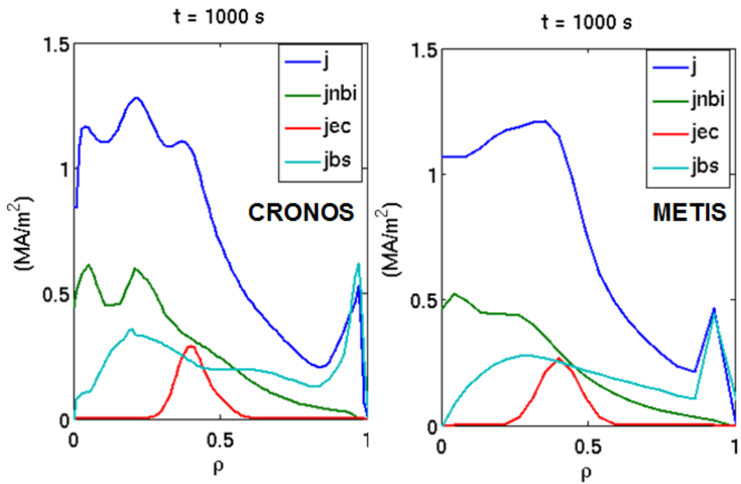
Figure 13: ITER hybrid scenario: computed current density profile and contributions from NBI, ECRH and bootstrap, in the flat-top phase. CRONOS (left) and METIS (right) simulations.
