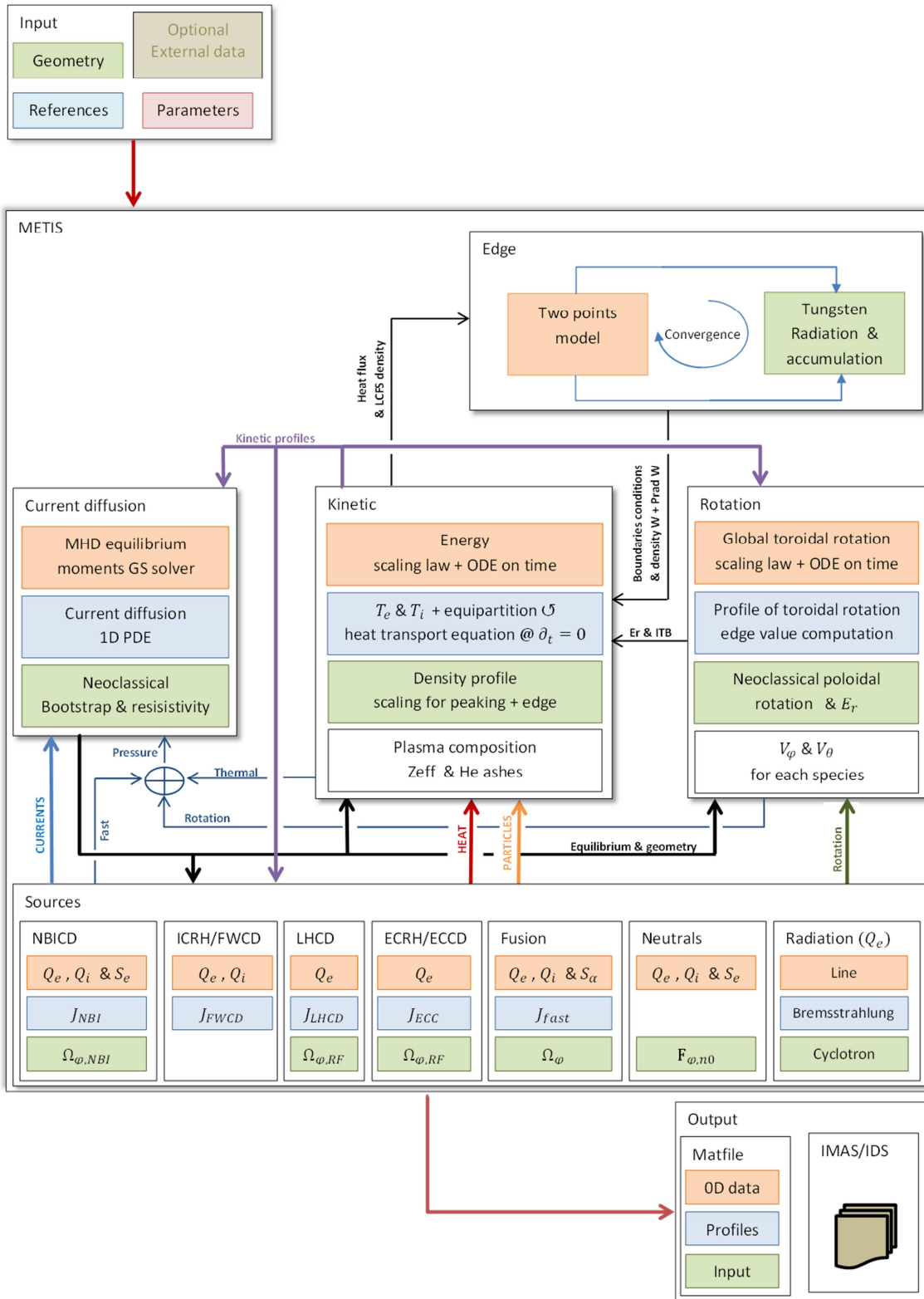
Figure 2: Overview of METIS internal organization
