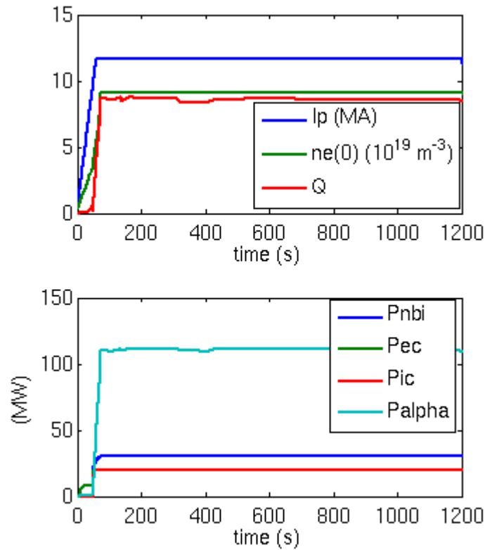
Figure 6: METIS simulation of ITER hybrid scenario: time evolution of various quantities, used as input waveforms or computed by METIS. Top: plasma current, central density and Q factor. Bottom: NBI, Ion Cyclotron, Electron Cyclotron and alpha powers. Note that Ion and Electron Cyclotron power waveforms are nearly superposed.
