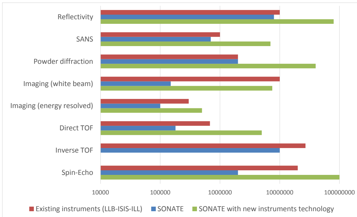
Figure 15: Comparison of the performances of different scattering techniques in terms of flux at the sample position ( \text{n}/\text{cm}^2/\text{s} ). (red) reference instruments at various facilities (LLB – ISIS – ILL) ; (blue) move of the existing instruments from Orphée to SONATE ; (green) performances after technical upgrades. The figures for the inelastic instruments (Direct TOF and Inverse TOF) have been provided by Jörg Voigt from JCNS.
