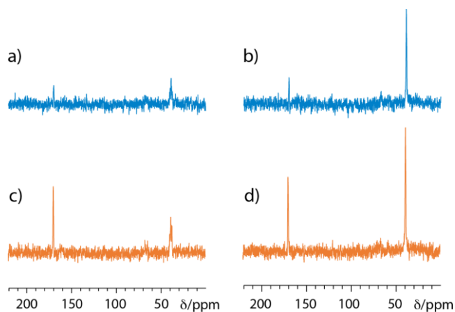
Figure 5. ^{13}\text{C} NMR spectra recorded in the same conditions with the WIFI-NMRS device on a 25-mM sample of ^{15}\text{N} - ^{13}\text{C} -enriched glycine in \text{D}_2\text{O} , in static mode (a) and b)) and with a gas flow of 1 mL/min (c) and d)). In b) and d) ^1\text{H} decoupling was applied during acquisition. An interscan delay of 1s was used for all these acquisitions. Other details: see the Supp. Info.
