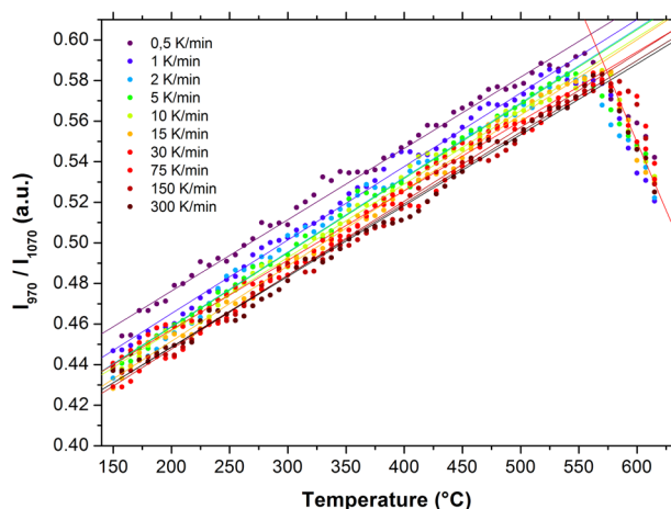
Fig. 3 Evolution of the intensity ratio of the fitted Raman band at 970 \text{ cm}^{-1} over one at 1070 \text{ cm}^{-1} as a function of temperature for ISG fibers cooled at different rates
