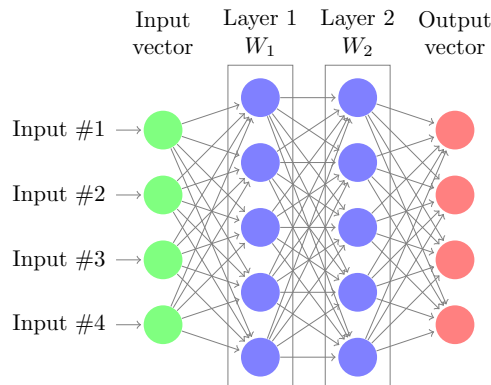
Figure 7. Graphical representation of layers
