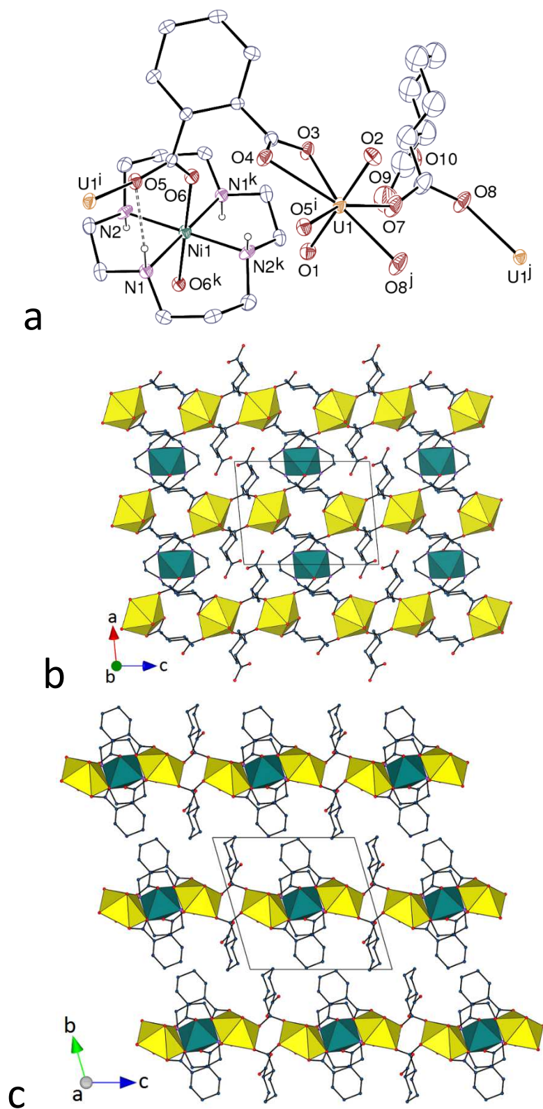
Figure 4. (a) View of compound 3. Displacement ellipsoids are drawn at the 20% probability level. Carbon-bound hydrogen atoms are omitted and the hydrogen bond is shown as a dashed line. Symmetry codes: i = 1 - x, 1 - y, 1 - z ; j = 1 - x, 1 - y, 2 - z ; k = 2 - x, 1 - y, 1 - z . (b) View of the 2D network. (c) Packing with sheets viewed edge-on.
