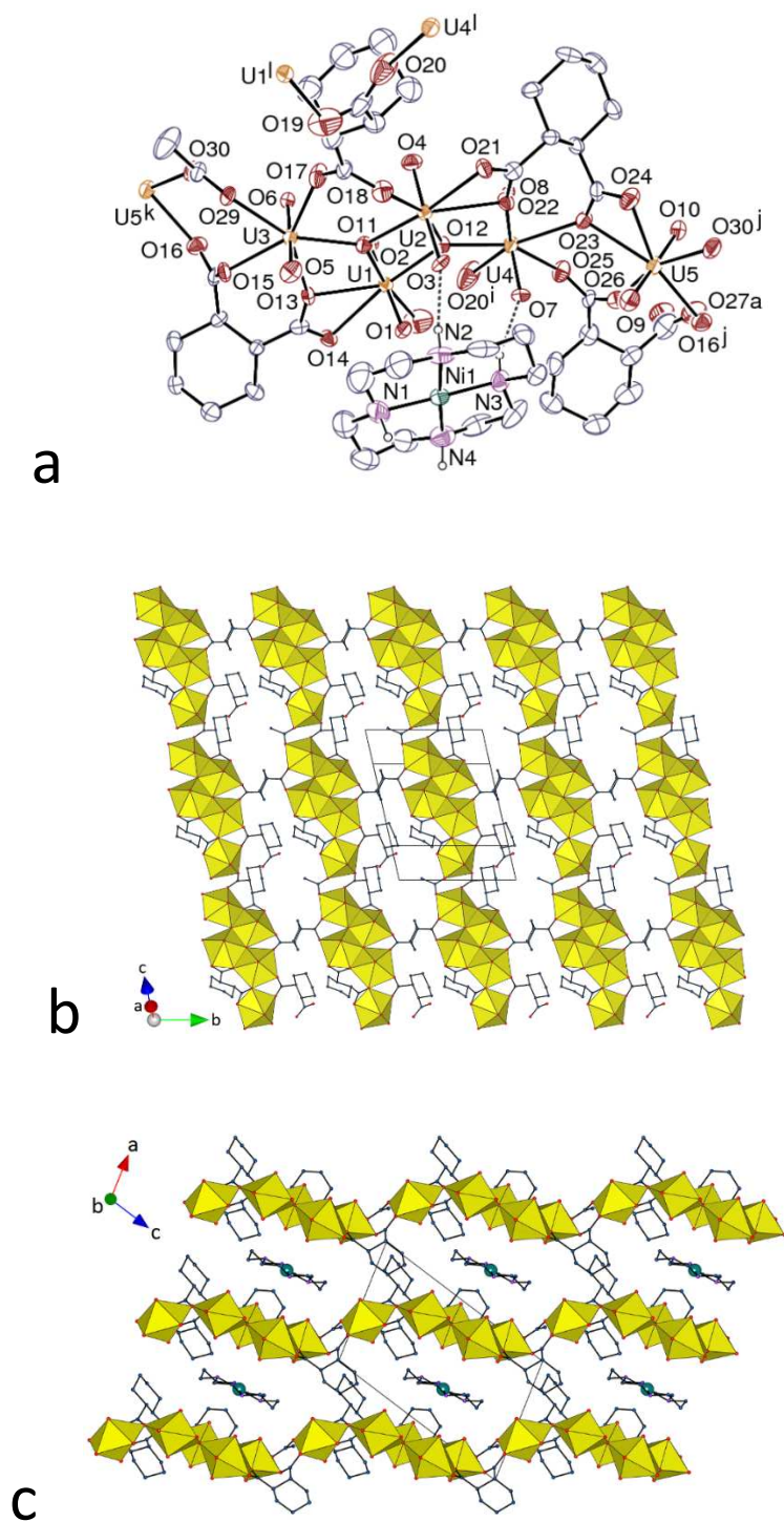
Figure 5. (a) View of compound 4. Displacement ellipsoids are drawn at the 30% probability level. Carbon-bound hydrogen atoms are omitted and hydrogen bonds are shown as dashed lines. Symmetry codes: i = x, y + 1, z ; j = x - 1, y, z - 1 ; k = x + 1, y, z + 1 ; l = x, y - 1, z . (b) View of the uranium-based 2D network. (c) Packing with layers viewed edge-on. Only one position of the disordered atoms is shown in all views.
