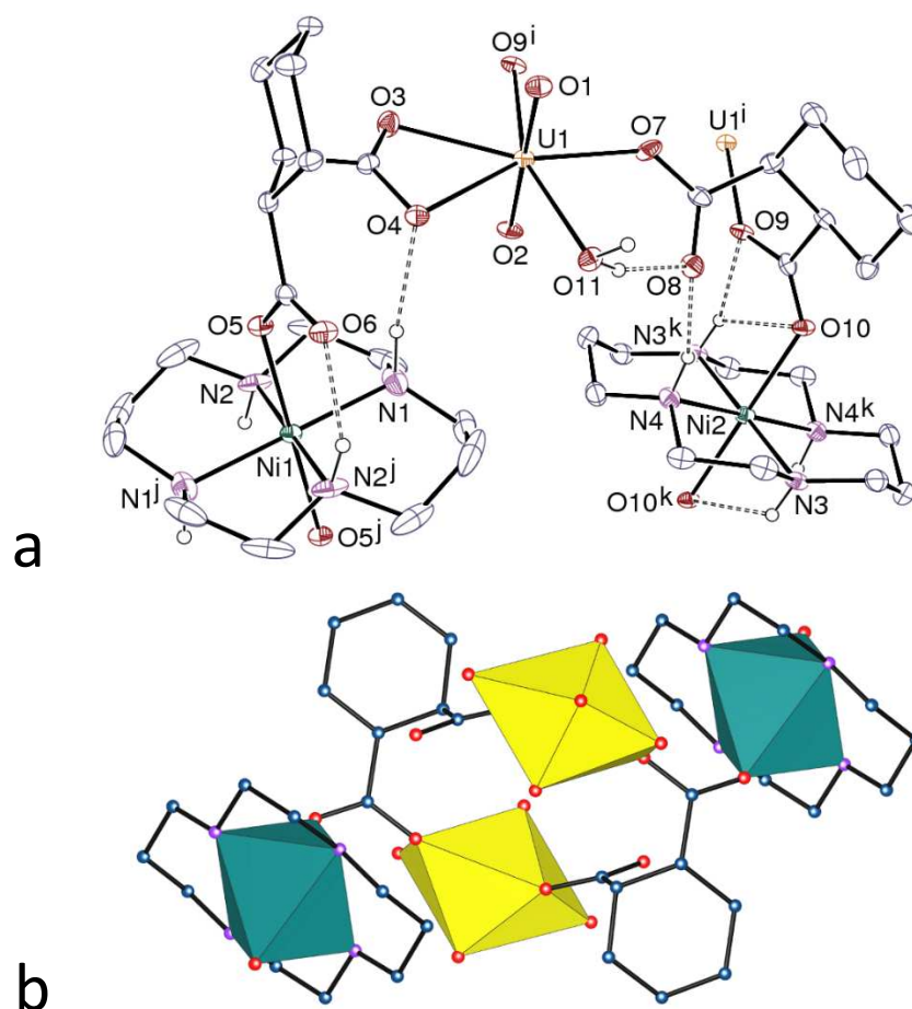
Figure 1. (a) View of compound 1 . Displacement ellipsoids are drawn at the 30% probability level. Carbon-bound hydrogen atoms are omitted and hydrogen bonds are shown as dashed lines. Symmetry codes: i = 1 - x, 1 - y, -z ; j = -x, 1 - y, 1 - z ; k = 1 - x, -y, -z . (b) View of the dimeric motif with uranium coordination polyhedra colored yellow and those of nickel(II) green, and hydrogen atoms omitted. For clarity, only two of the four surrounding \text{Ni}^{\text{II}} cations are shown.
