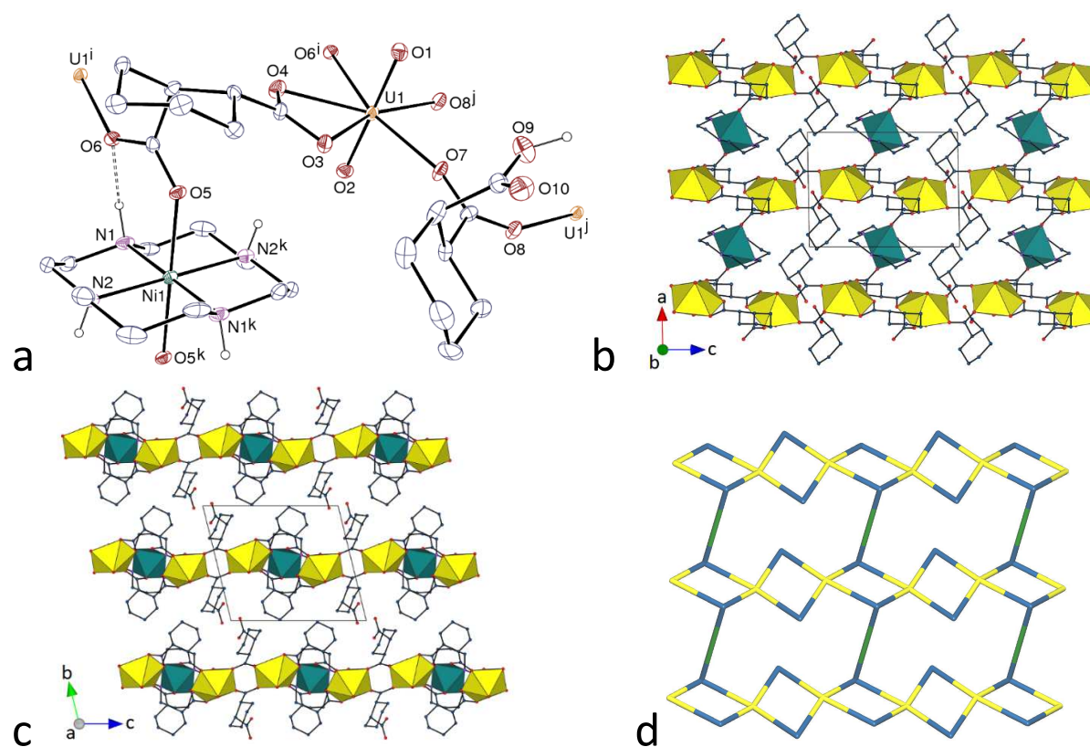
Figure 3. (a) View of compound 2 . Displacement ellipsoids are drawn at the 20% probability level. Carbon-bound hydrogen atoms are omitted and the hydrogen bond is shown as a dashed line. Symmetry codes: i = 1 - x, 1 - y, 1 - z ; j = 1 - x, 1 - y, 2 - z ; k = 2 - x, 1 - y, 1 - z . (b) View of the 2D network. (c) Packing with sheets viewed edge-on. (d) Representation of the 2D network (yellow: uranium nodes; blue: centroids of the dicarboxylate ligand nodes or edges; green: nickel links).
