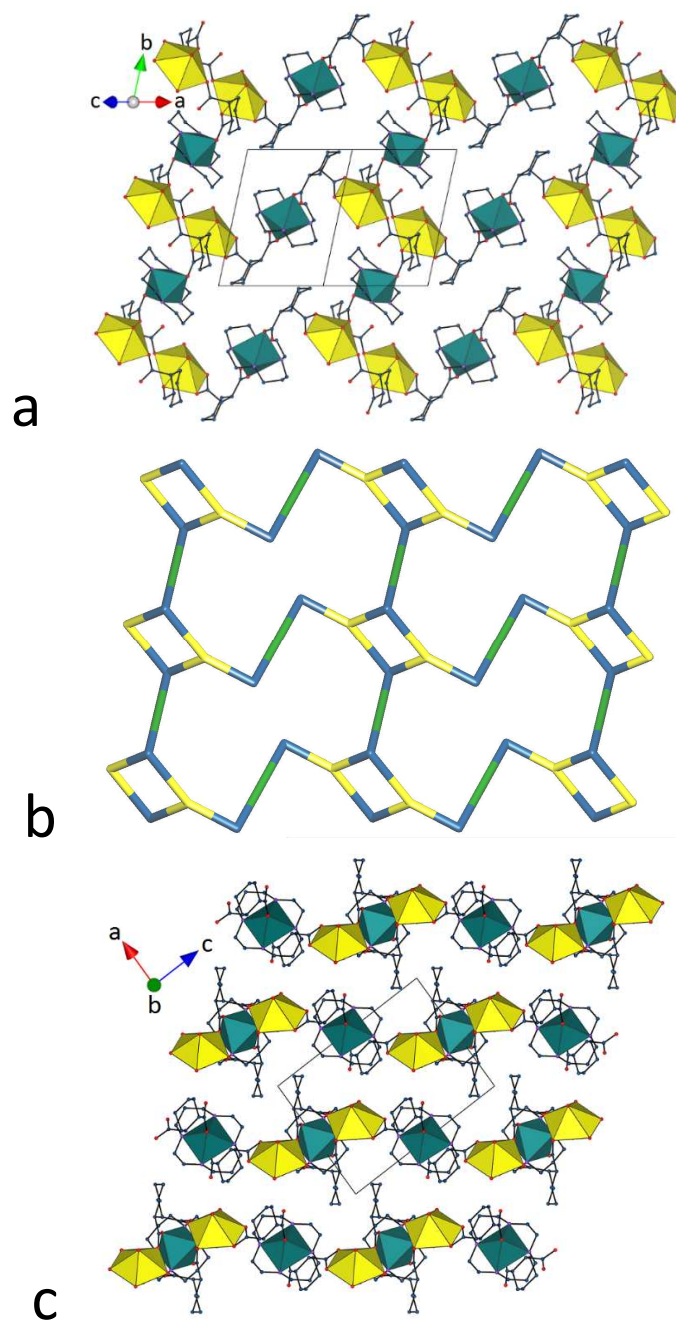
Figure 2. (a) View of the 2D network in compound 1 . (b) Representation of the 2D network (yellow: uranium nodes; blue: centroids of the dicarboxylate ligand nodes or links; green: nickel links). (c) View of the packing with layers viewed edge-on.
