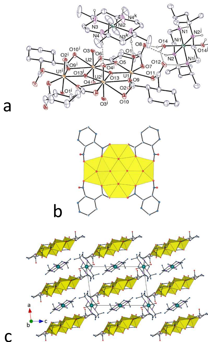
Figure 6. (a) View of compound 5 . Displacement ellipsoids are drawn at the 20% probability level. Carbon-bound hydrogen atoms are omitted and hydrogen bonds are shown as dashed lines. Symmetry codes: i = 1 - x, 1 - y, 1 - z ; j = -x, 1 - y, -z ; k = -x, 1 - y, 1 - z . (b) View of the anionic tetranuclear uranyl complex. (c) View of the packing. Only one position of the disordered atoms is shown in all views.
