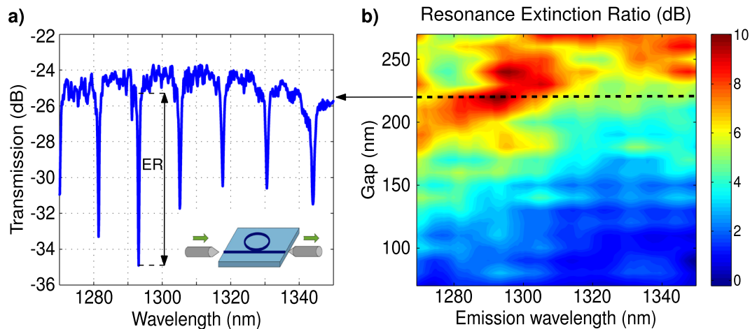
Figure 3. Measured linear spectral response for TM mode of Si micro-ring resonators with bus waveguide width of W_{bus} = 270 nm, ring waveguide width of W_{ring} = 350 nm, ring radius of R = 5 \mu\text{m} for (a) fixed bus-to-ring gap of G = 220 nm, and (b) bus-to-ring gap varying between 80 nm and 270 nm. Dashed line indicates position of spectrum for gap G = 220 nm, shown in (a).
