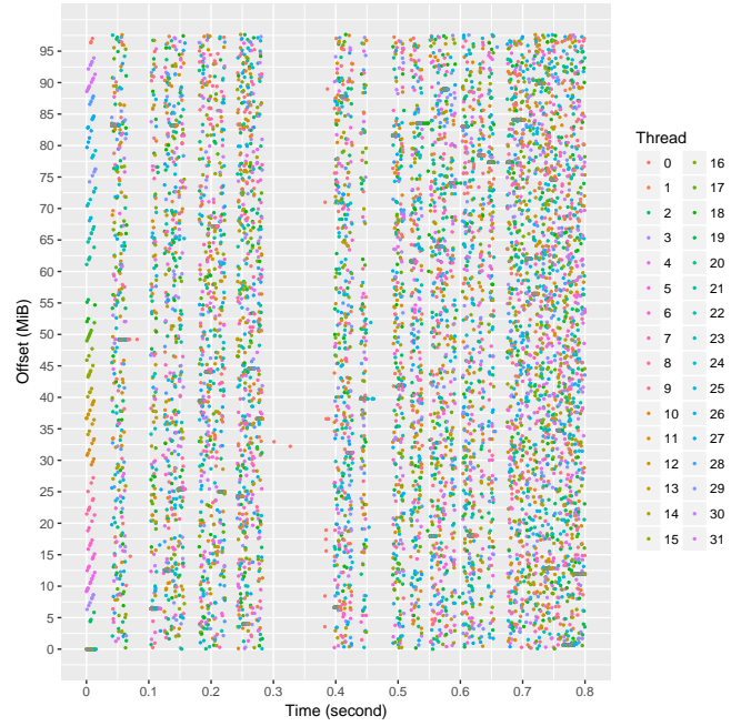
Figure 5: Evolution over time of, per thread, memory accesses to the pages of the block object in Streamcluster. The pattern shown here over 0.8 seconds is repeated over all the iterations of the kernel.
