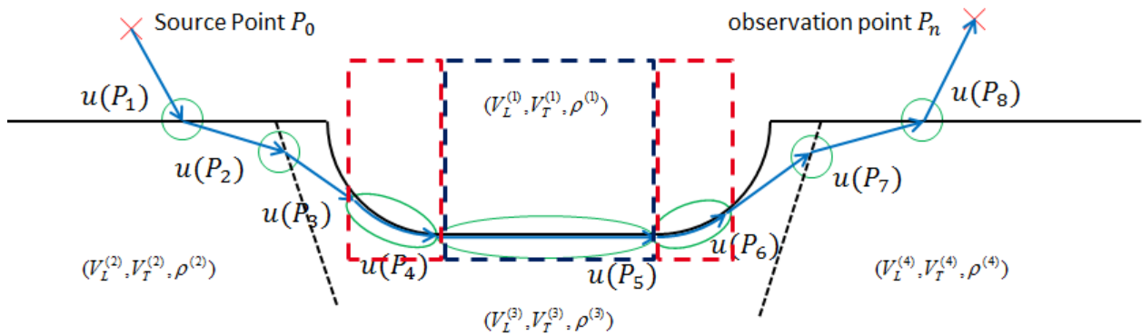
FIGURE 7 Amplitude calculation along a ray path calculated by GIRT over a scoured irregularity. Red dashed blocks: creeping ray along cylindrical parts. Blue dashed block: grazing ray along the planar part.
