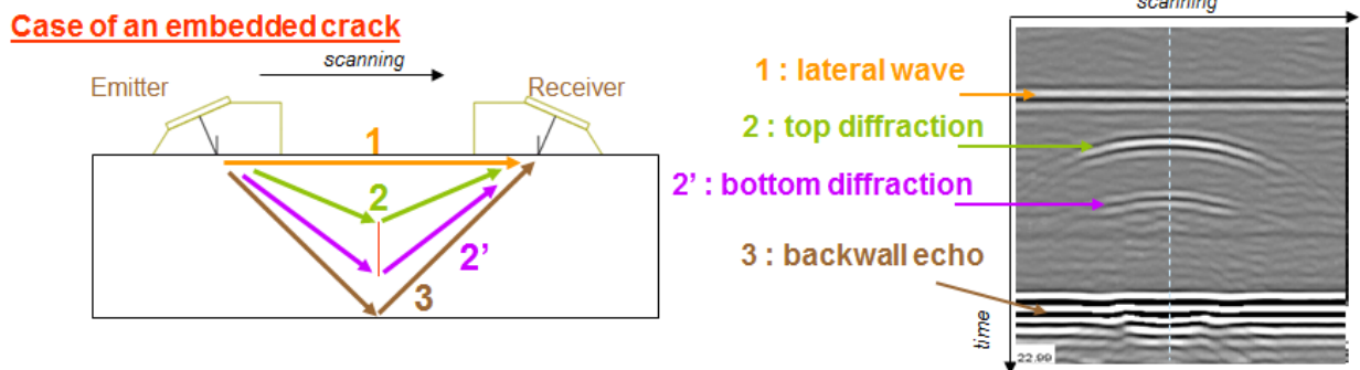
FIGURE 1. Illustration of TOFD inspection technique over a planar specimen and related echoes for an embedded crack
