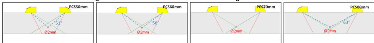
FIGURE 11: SDH at 20mm depth, ray path display and value of the direct ray incidence angle on the SDH. TOFD inspection, contact probe Ø6.35mm, 5MHz, P60°, various PCS.
