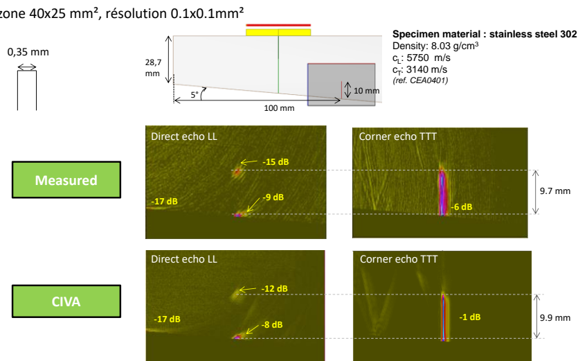
FIGURE 14. simulated and experimental TFM images obtained on the 10mm height notch with the 5° slope.
