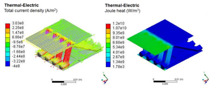
Fig. 6 Results of current density and Joule heat ( R_c=1\text{m}\Omega )
