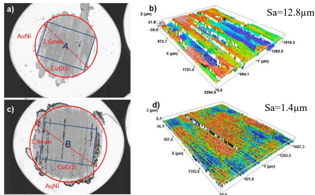
Fig. 16 SEM and confocal topography of the worn pins: a). SEM image of the original pin; b). Confocal image of zone A; c). SEM image of the thermal aged pin; b). Confocal image of zone B.
