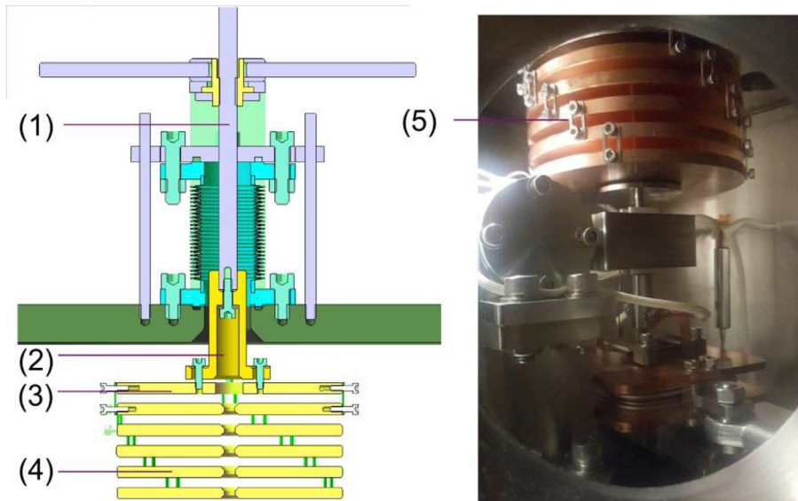
Fig. 3. Loading system of the HV-MTEST: (1). Load lifting mechanism; (2). Al 2 O 3 insulation joint; (3). Dead load support; (4). Dead load plates (6 N × 5); (5). Hooks (× 16).
