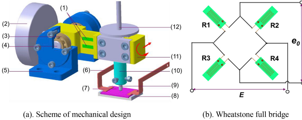
Fig. 2. Design of the CoF measurement system: (1). Strain gauges (× 4); (2). Counterweight; (3). Bearings (× 2); (4). Central shaft; (5). Beam support; (6). Electrodes (× 2); (7). Plate sample; (8). AlN ceramic plate; (9). Pin sample; (10). Pin sample holder; (11). Cantilever beam; (12). Loading support.
