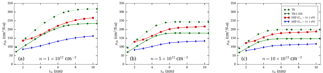
FIG. 10. Hole mobility in Si films. Comparison between TB-KG calculations (green circles) and KP-NEGF calculations with \Xi_{ac}^h = 10.2 eV (red squares) and \Xi_{ac}^h = 15.5 eV (blue lozenges). (a) n = 10^{12} cm ^{-2} ; (b) n = 5 \times 10^{12} cm ^{-2} ; (c) n = 10 \times 10^{12} cm ^{-2} . The green dotted lines are the original TB values, while the green solid lines are rescaled by a factor 1/1.356 in order to account for the difference between the experimental and TB-KG bulk mobility.
