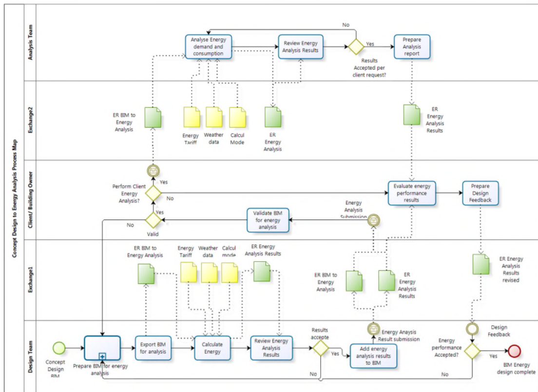
Figure 5 The Energy Analysis Process Map
