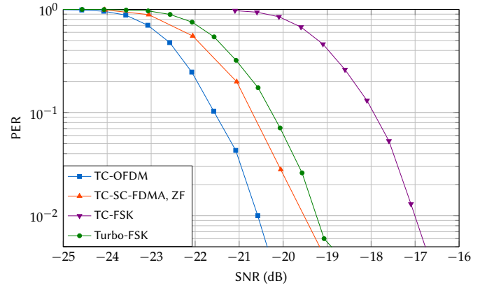
Figure 5: Performance of the four compared solutions under Rayleigh fading channel with ETU profile. The relative speed is equal to 50\text{km}\cdot\text{h}^{-1} and the carrier frequency is set to 2.5GHz.
