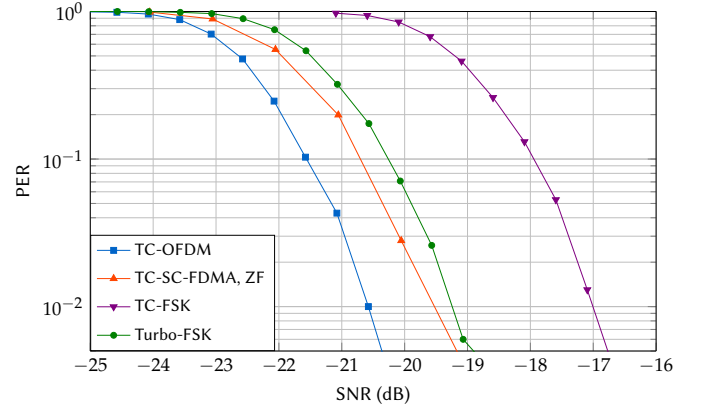
Figure 5: Performance of the four compared solutions under Rayleigh fading channel with ETU profile. The relative speed is equal to 50 \text{ km} \cdot \text{h}^{-1} and the carrier frequency is set to 2.5 \text{ GHz} .
