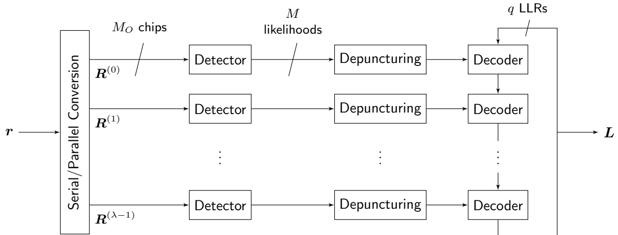
Figure 5: The C-TFSK receiver architecture.
