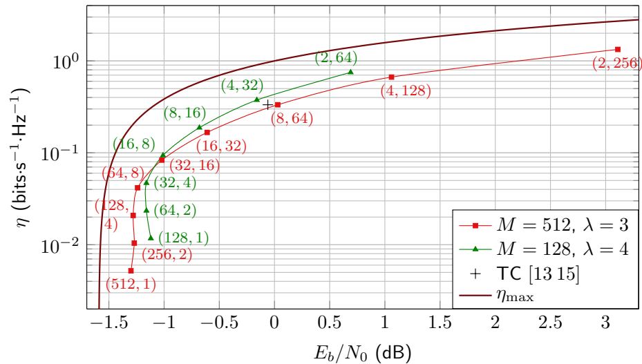
Figure 16: Spectral efficiency versus threshold for various sizes of alphabet M and parameter \lambda , using various combinations of (M_O, M_L) . The spectral efficiency is computed with (8). The maximum achievable spectral efficiency according to the channel capacity is computed using (1). A X mapping was selected, without any puncturing (i.e. R_p = 1 ).
