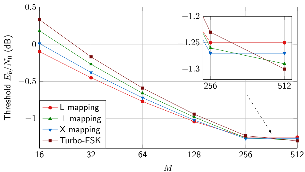
Figure 12: Thresholds for various size of alphabet M and mappings, with M_L = 4 (QPSK) and \lambda = 3 .
