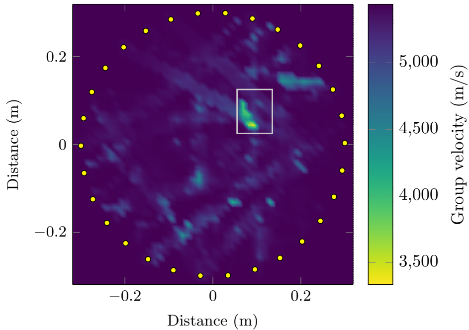
Figure 8 : Passive time-of-flight tomography using the Simultaneous Algebraic Reconstruction Technique (SART [6, page 275])
