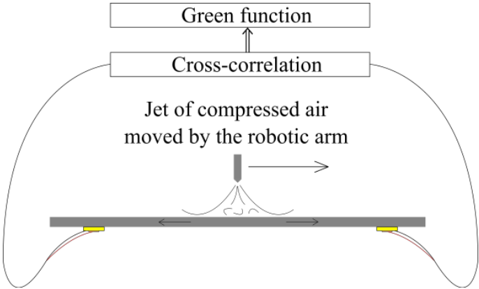
Figure 4 : Process of acquisition for passive tomography
