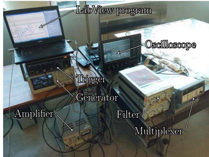
Figure 1 : Material composing the bench
