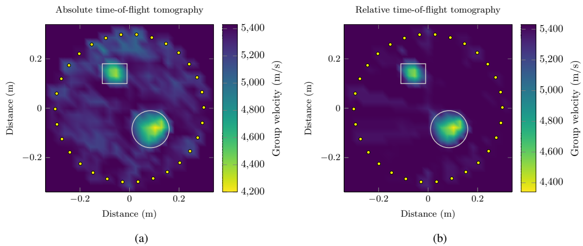
Figure 6 : Active time-of-flight tomography using the Simultaneous Algebraic Reconstruction Technique (SART [6, page 275])
