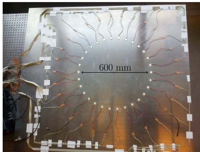
Figure 2 : 30 piezoelectric transducers ( \varnothing 18 mm) glued on the 2 mm thick aluminum plate
