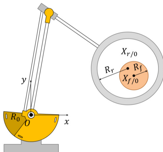
Figure 2: 2DoF ETHD with ring center X_{r/0} and finger center X_{f/0} (adapted from (Gonzalez, 2015)).
