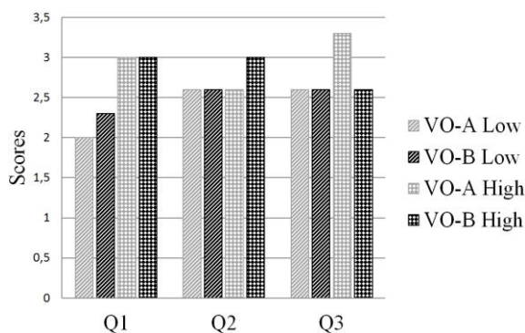
Figure 18: Survey scores.
