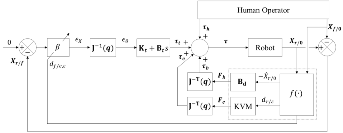
Figure 7: Offset transition-based control. KVM:interaction force. f(\cdot) : estimation of the robot's end-effector speed \dot{X}_{r/o} with negative sign and of the distance d_{f/\epsilon} .
