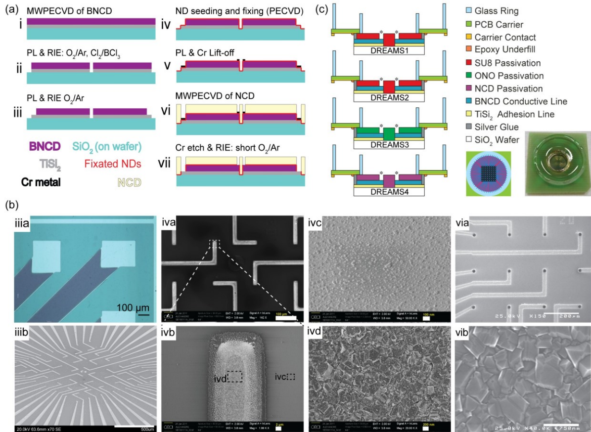
Figure 2. a) NCD-passivated BNCD/TiSi 2 MEA fabrication. PL: photolithography, MWPECVD: microwave plasma enhanced chemical vapour deposition, RIE: reactive ion etching. (b) Images of MEA corresponding to the process steps in (a). (iii.a) Optical image of exposed TiSi 2 bondpads and BNCD feedlines, scale bar 100 μm. (iii.b) Scanning Electron Microscope (SEM) image of MEA prior to passivation, scale bar 500 μm. (iv.a) SEM of MEA post-ND-seeding and MWPECVD fixation, scale bar 100 μm (iv.b) Enlarged image of an electrode, scale bar 2 μm. (iv.c) SEM image of NDs seeded on the SiO 2 substrate, scale bar 100 nm and (iv.d) on the BNCD electrode, scale bar 200 μm, as labelled in (iv.b). (vi.a) MEA post-NCD MWPECVD growth, with electrodes covered by Cr caps, scale bar 200 μm. (vi.b) Magnification of NCD grown over the SiO 2 substrate, confirming the NCD nature of the material, scale bar 750 nm. (C) Schematic cut through of packaged chips with electrode openings marked (*), including a schematic top view of the packaged BNCD electrode array and a photograph of the final MEA device.
