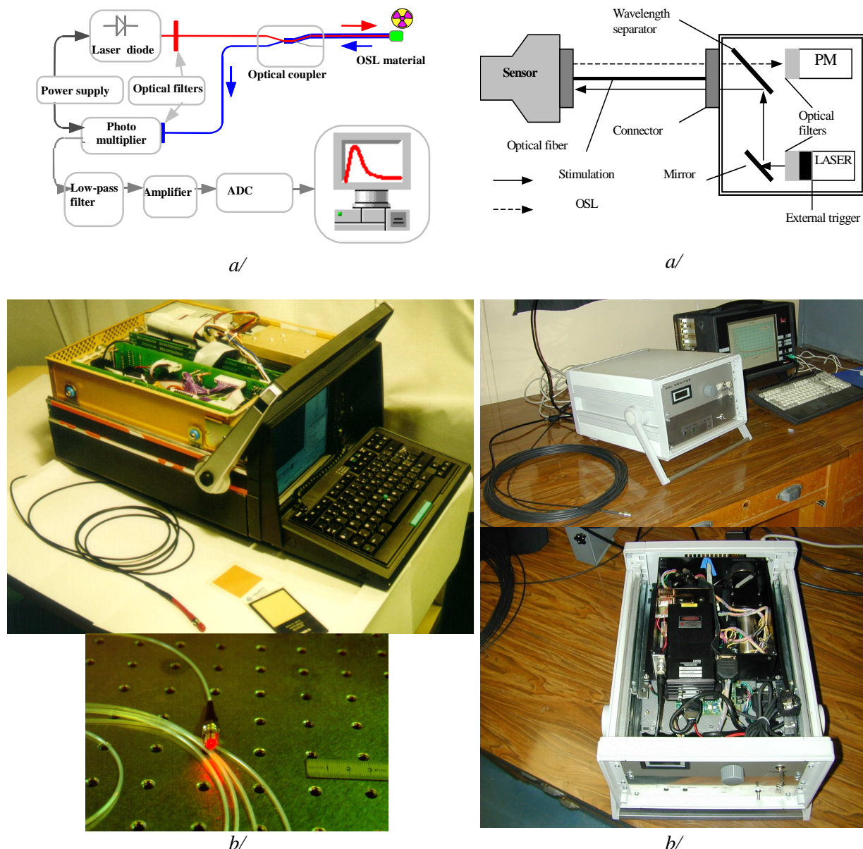
FIG. 2 : First generation of OSL optoelectronic dosimeters (OSL 1) a/ OSL 1 : Scheme of operation b/ View of the PC-based system and fiber-connected OSL transducer
