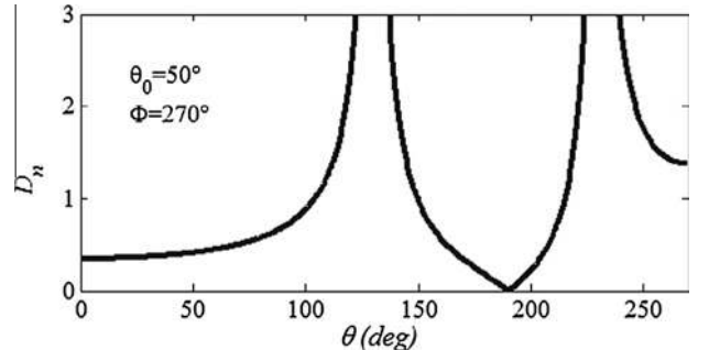
Fig. 2. GTD diffraction coefficient for \Phi = 270^\circ and \theta_0 = 50^\circ . \omega = 2\pi \cdot 1 MHz and c = 2472 m/s.
