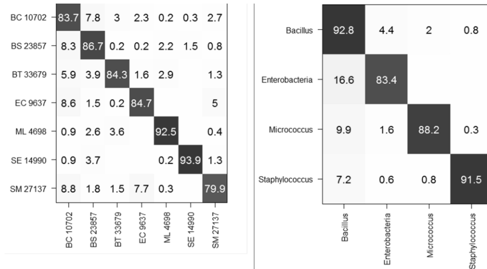
Figure 9. Mean confusion matrix using 10 s acquisition time and SVM classification technique. Left) species level classification (86.5 % ± 0.5 %) and Right) families level classification (89 % ± 0.5 %).
