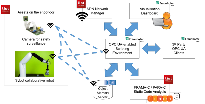
Fig. 1. Systems architecture for the runtime deployment of functionality. Dashed lines denote wireless connectivity based on the NEON SDN framework. Blue arrows denote either communication via OPC UA or local inter-process communication.
