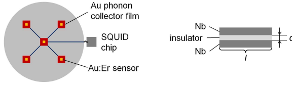
Fig. 1 (Color online) Left: Basic design of a LUMINEU light detector with several small area MMCs and planar readout coils connected in series and additional phonon collector films. Right: Low inductance niobium-insulator-niobium strip line.
