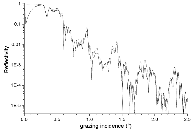
Fig. 3 Reflectance at Cu K_\alpha line of the flat reflectivity profile sample. The solid line represents the measured data and the dotted line is the calculation with a 1.3% thickness correction on the Mo layers
