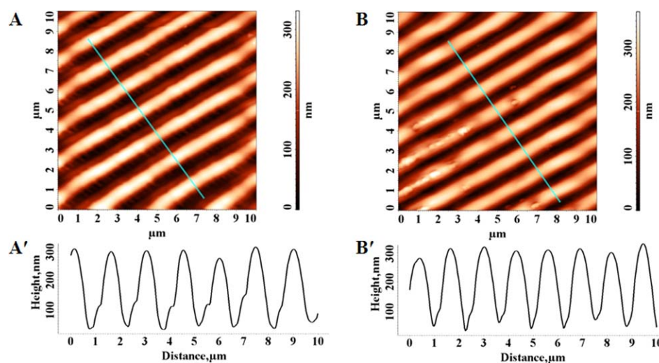
Figure 4. AFM images of the SRG corresponding to sample 3: (A) laser fluence of 14 \text{mJ}/\text{cm}^2 and 200 pulses (relief amplitude = 300 nm) and (B) laser fluence of 16.5 \text{mJ}/\text{cm}^2 and 200 pulses (relief amplitude = 300 nm). The film thickness was 500 nm, and the SRG periodicity was 1.4 \mu\text{m} . [Color figure can be viewed in the online issue, which is available at wileyonlinelibrary.com .]
