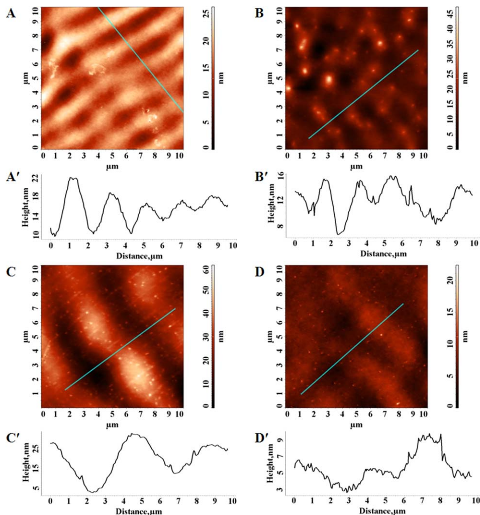
Figure 2. AFM images of the SRGs corresponding to sample 2 registered 14 days after inscription: (A) fluence of 14 mJ/cm 2 and 100 pulses, (B) fluence of 8.8 mJ/cm 2 and 100 pulses, (C) fluence of 13.8 mJ/cm 2 and 100 pulses, and (D) fluence of 11.8 mJ/cm 2 and 100 pulses. The film thicknesses were (A,B) 500 and (C,D) 1000 nm. [Color figure can be viewed in the online issue, which is available at wileyonlinelibrary.com .]
