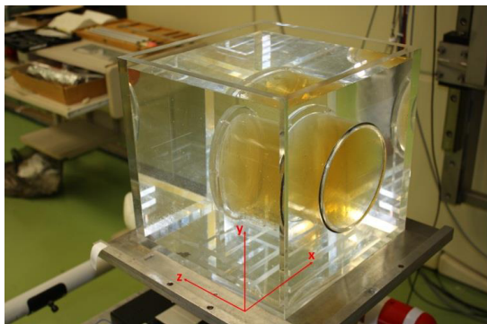
Figure 6: View of gel cylinder irradiated in a 30x30x30 cm 3 water phantom in front of a 6 MV LINAC photon beam.
