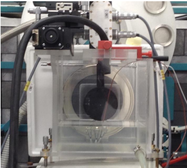
Figure 1: The mixed graphite-water ENEA calorimeter.
