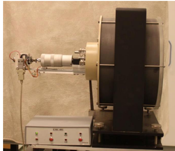
Figure 2: The MKEH extrapolation chamber
