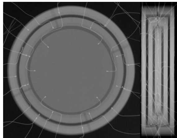
Figure 3: Top and side radiography of the LNE-LNHB graphite calorimeter detector.
