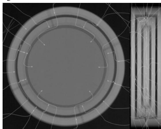
Figure 3: Top and side radiography of the LNE-LNHB graphite calorimeter detector.
