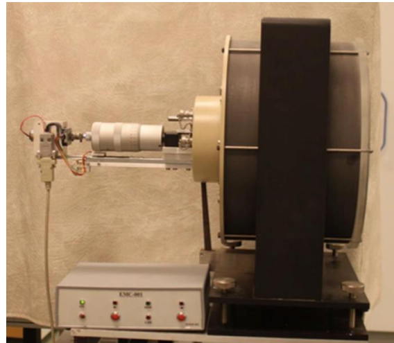
Figure 2: The MKEH extrapolation chamber
