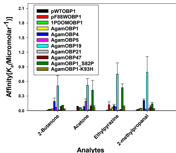
Figure 1: Affinity constants of the screened OBP1s toward the selected signature volatiles of tobacco, determined in the liquid phase using a fluorescent probe and competitive ligand binding.
